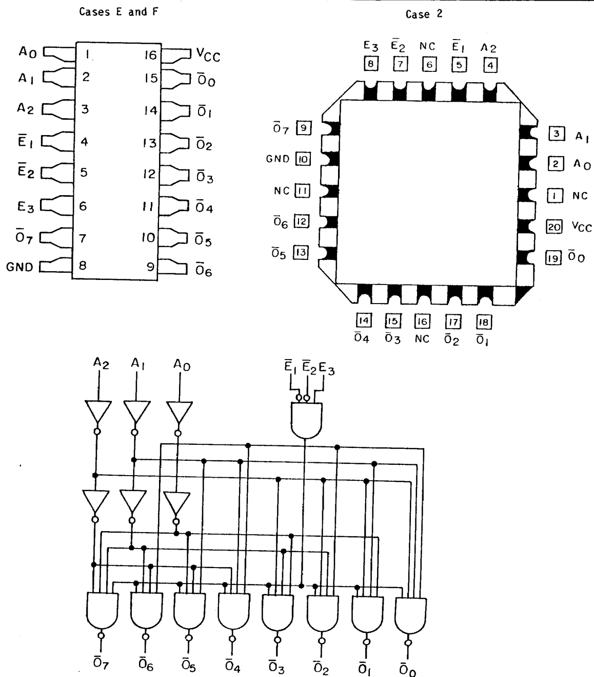
FIGURE 1. Logic diagram and terminal connections.
