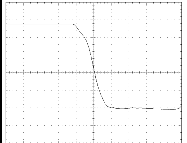
Pulse Fall Time: 13ns at 950V 10ns/Div horizontal scale, 200V/Div vertical scale
