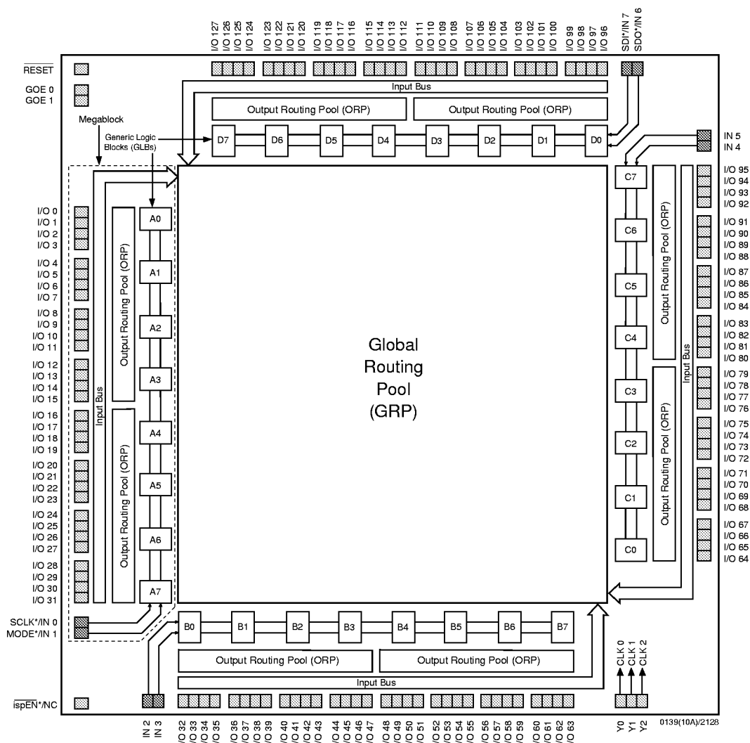
Figure 1. ispLSI and pLSI 2128 Functional Block Diagram
