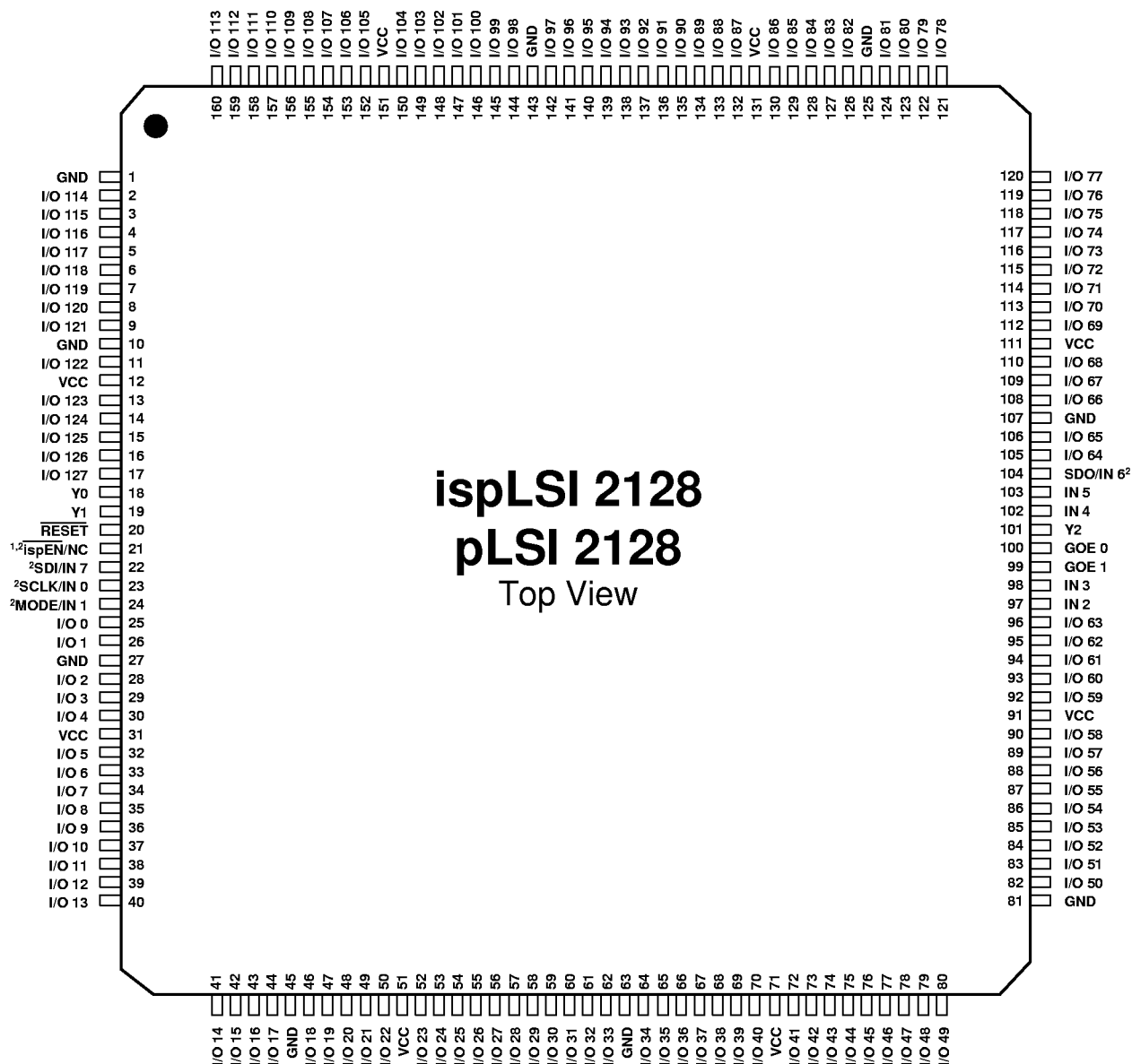
ispLSI and pLSI 2128 160-Pin PQFP Pinout Diagram
