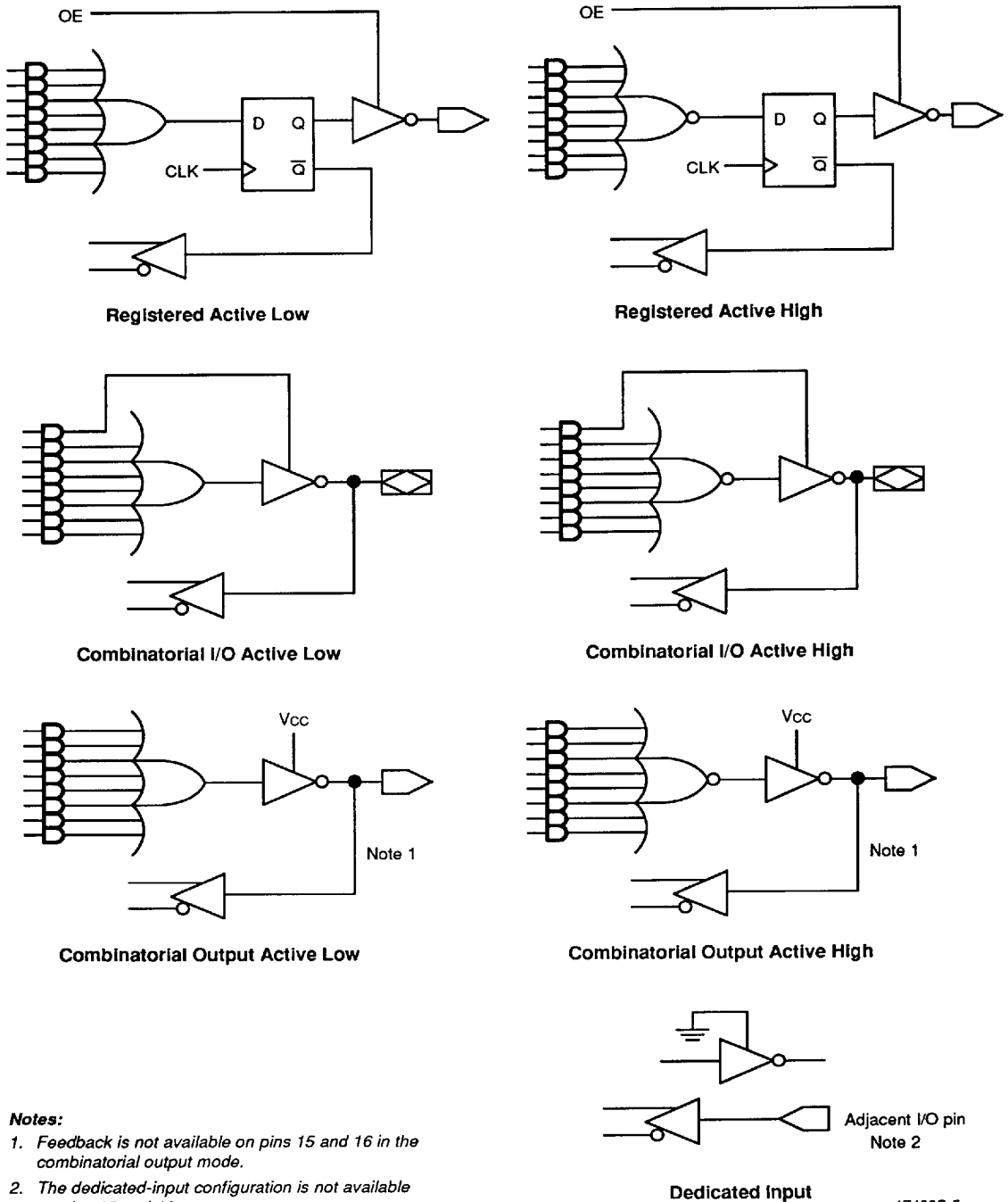
Figure 2. Macrocell Configurations
