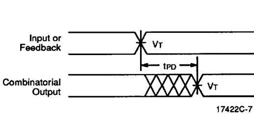
Combinatorial Output
