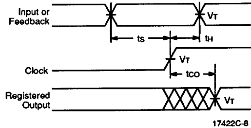
Registered Output
