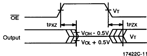
OE to Output Disable/Enable
