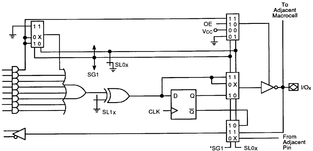
Figure 1. PALLV16V8Z Macrocell
