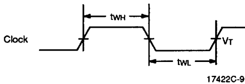
Clock Width
