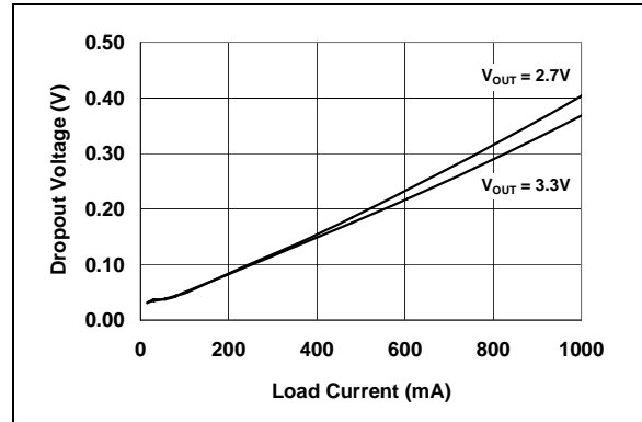
FIGURE 2-4: Dropout Voltage vs. Load Current.
