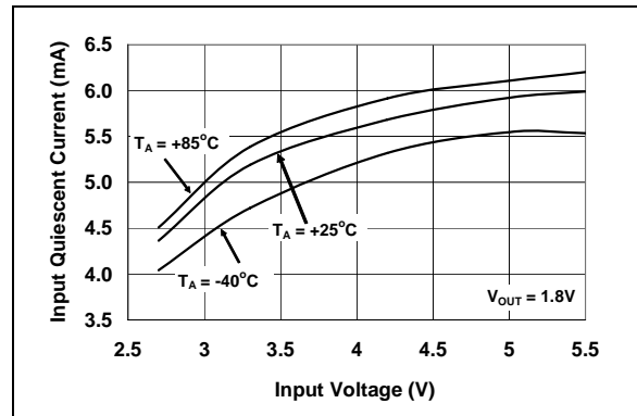
FIGURE 2-5: Input Quiescent Current vs. Input Voltage.
