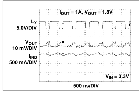
FIGURE 2-14: High Load Current Switching Waveform.
