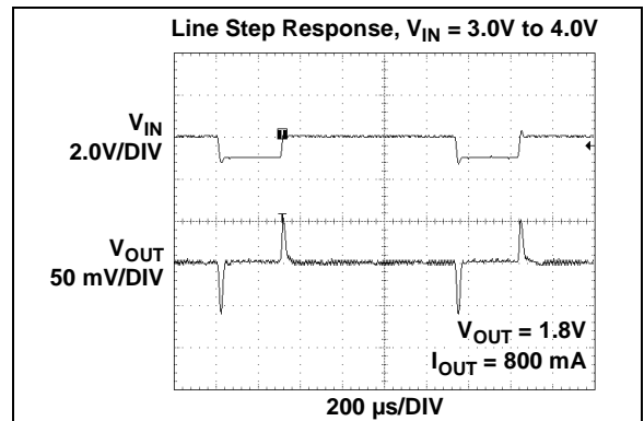
FIGURE 2-11: Line Transient Response.
