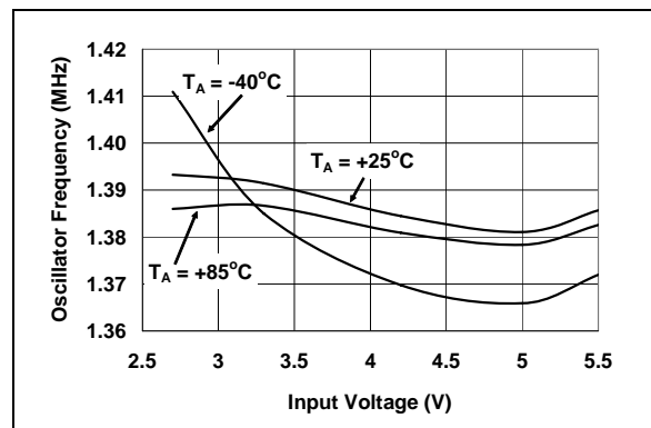
FIGURE 2-6: Oscillator Frequency vs. Input Voltage.
