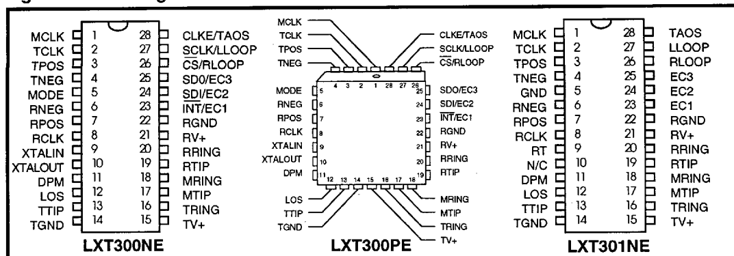
Figure 1: Pin Assignments
