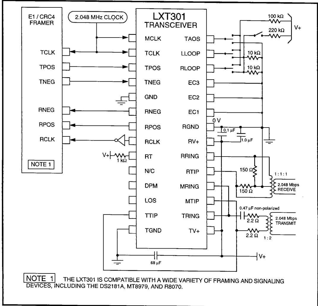
Figure 8: Typical LXT301 75 \Omega E1 Application
