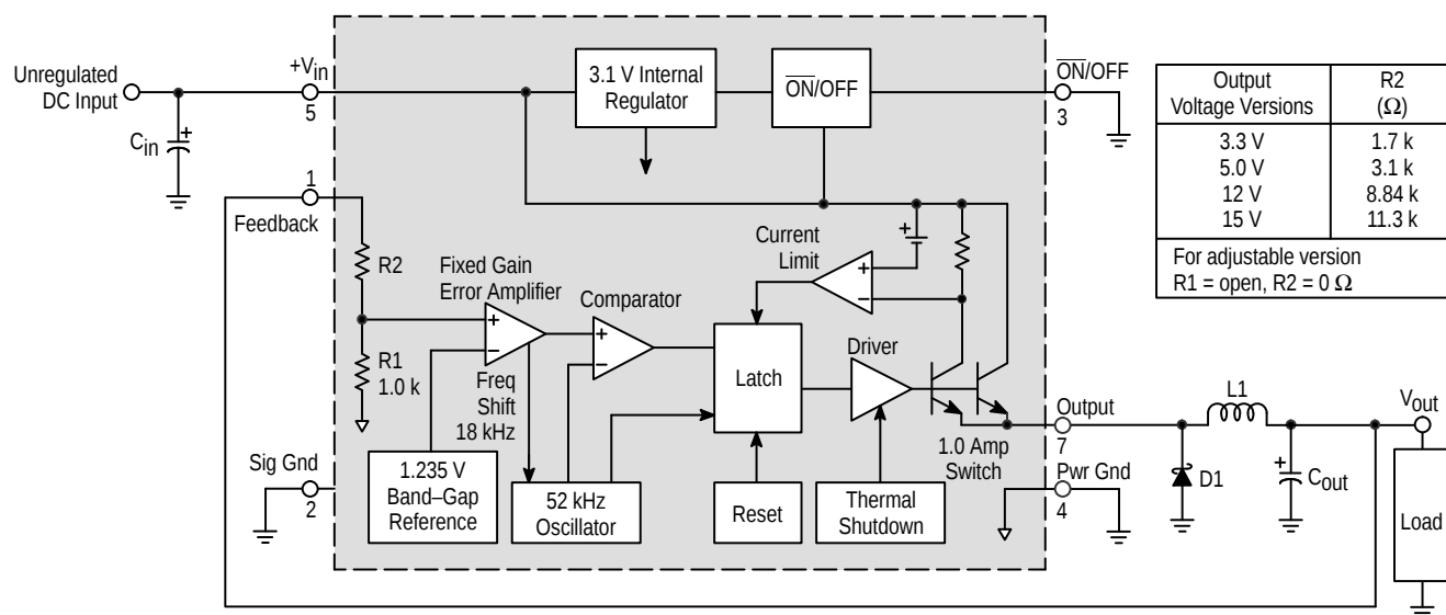
Representative Block Diagram and Typical Application
