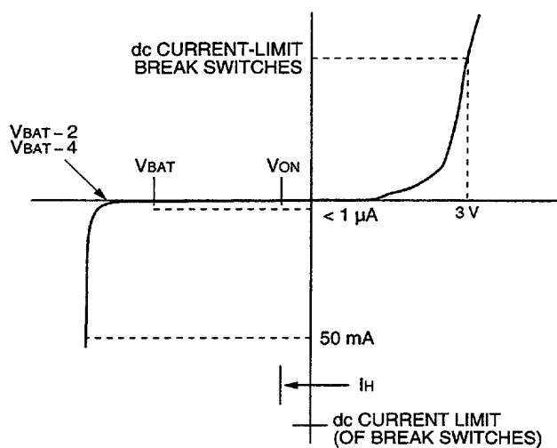
Figure 3. Protection Circuit A Version
