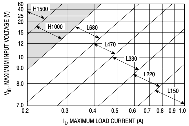
Figure 18. LM2575-5.0
