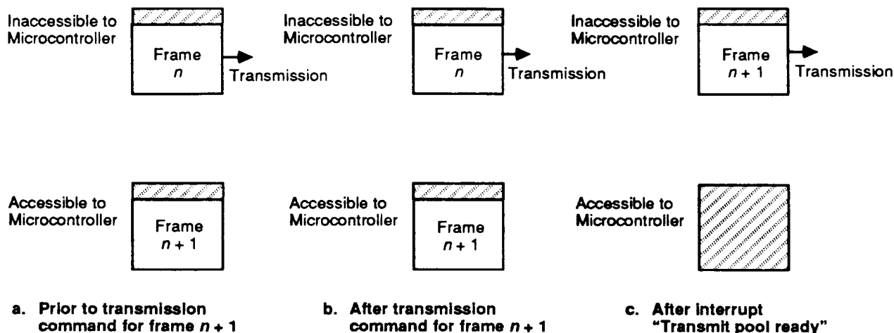
Figure 8. Transmit FIFO
