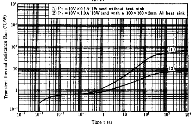
R_{th(t)} - t
