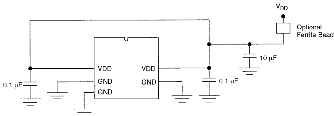
Figure 1. Recommended Circuit Configuration
