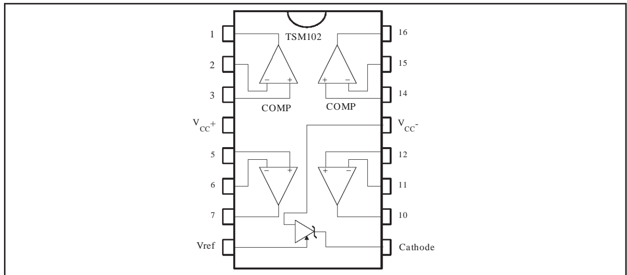
Figure 1: TSM102 Pinout
