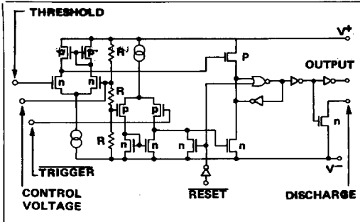
Figure 5. Equivalent circuit.
