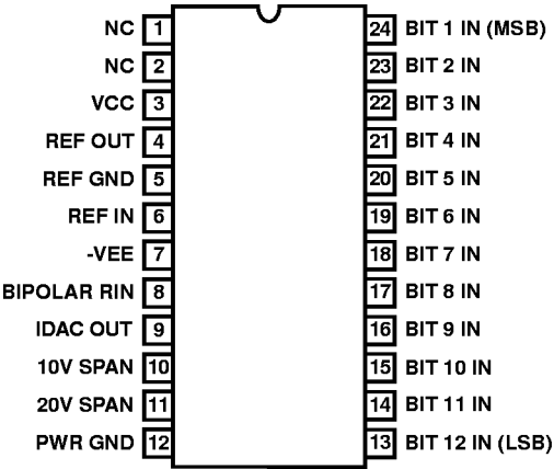
HS1-565ARH MIL-STD-1835 CDIP2-T24 (SBDIP) TOP VIEW
