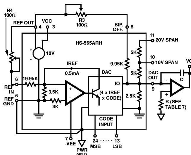
FIGURE 4. BIPOLAR VOLTAGE OUTPUT
