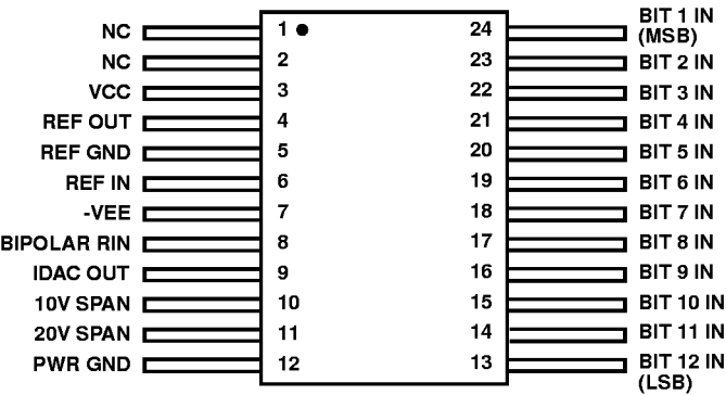
H59-565ARH MIL-STD-1835 CDFP4-F24 (CERAMIC FLATPACK) TOP VIEW
