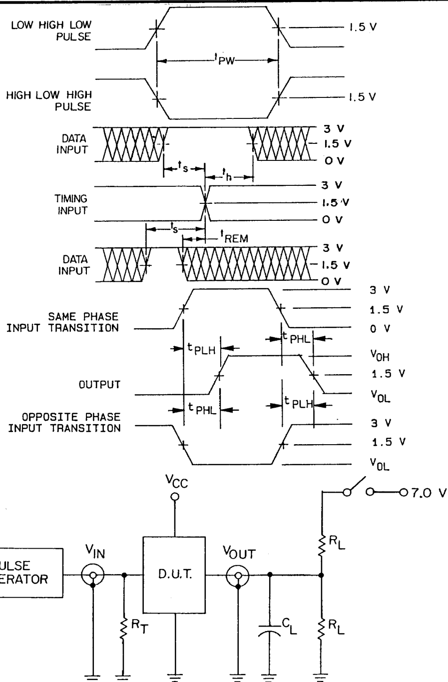
FIGURE 4. Switching waveforms and test circuit.
