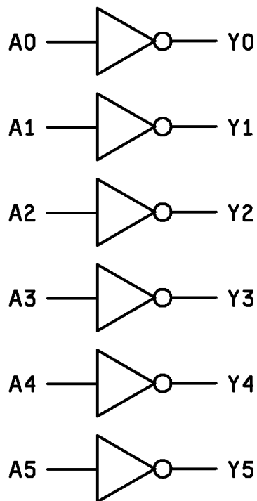
FIGURE 3. Logic diagram.
