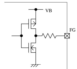
Fig. 2 Equivalent around FG
