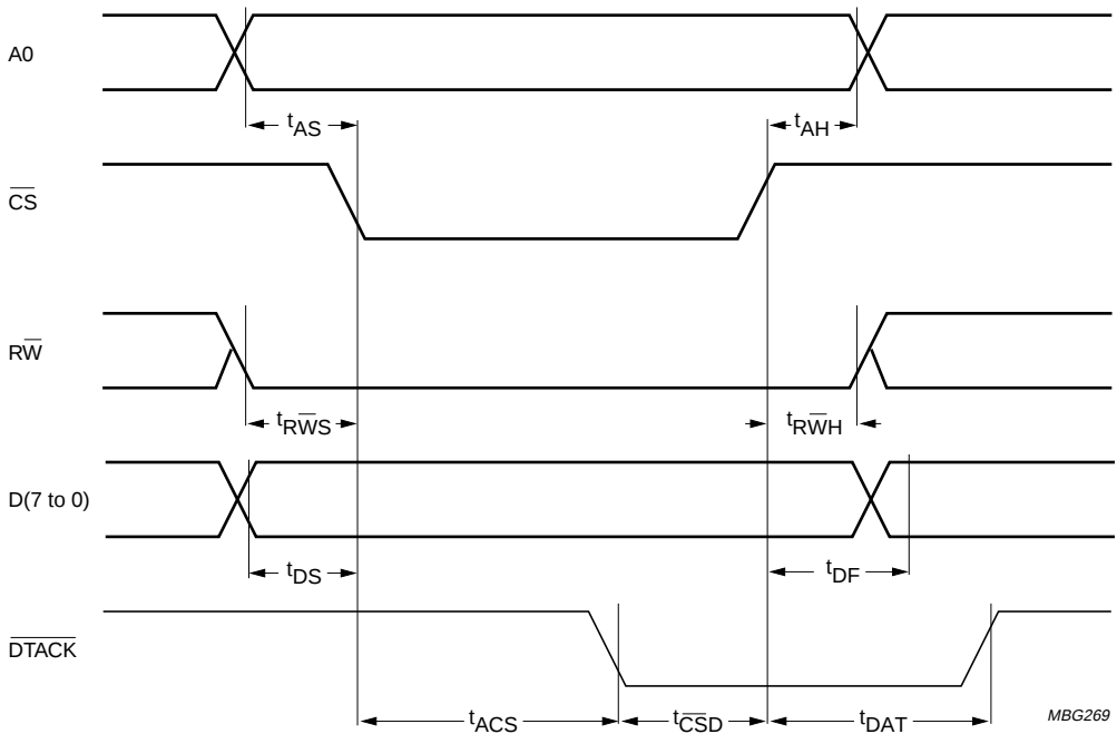
Fig.11 MPU interface timing (write cycle).
