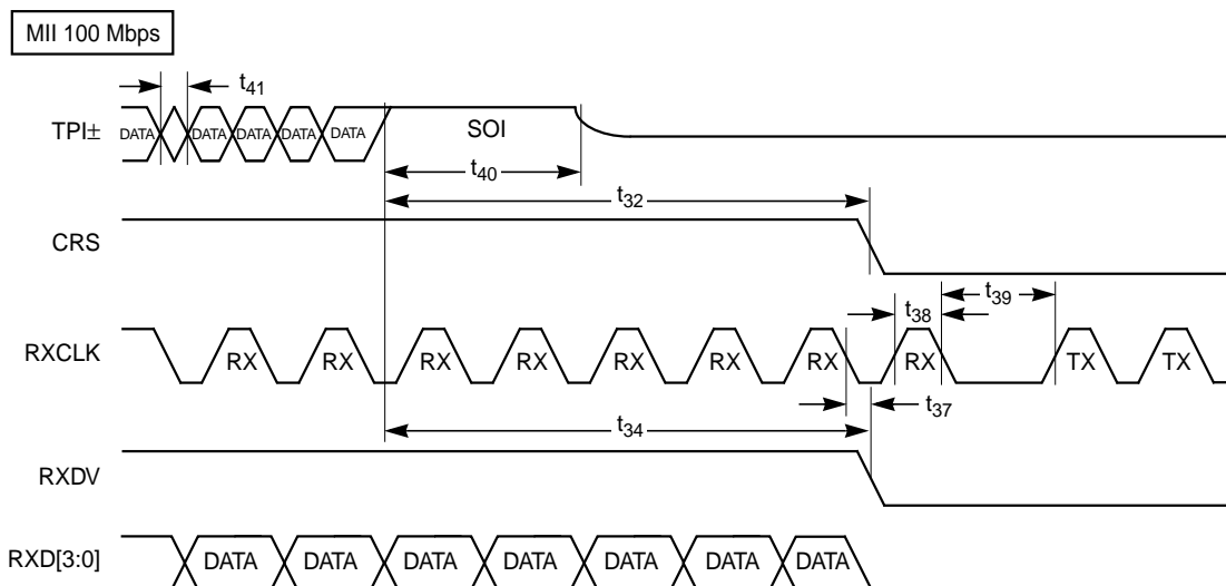
Figure 25 Collision Timing, Receive
