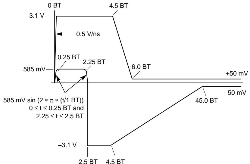
Figure 6 SOI Output Voltage Template - 10 Mbps
