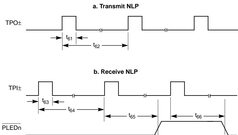
Figure 28 NLP Link Pulse Timing
