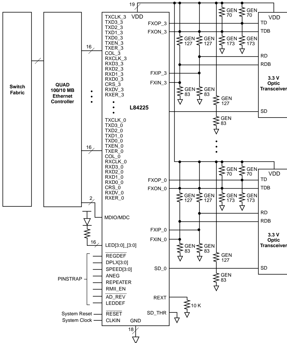
Figure 12 Typical Switching Hub Port Schematic Using the L84225 in FX Mode with 3.3 V Transceivers
