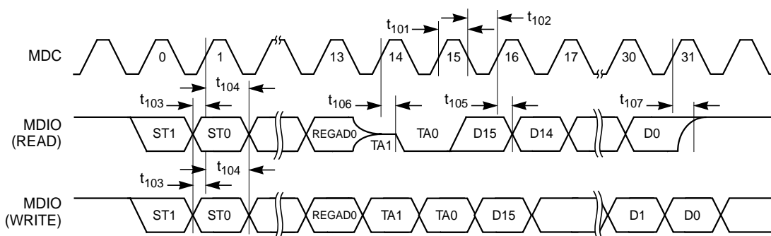
Figure 32 MI Serial Port Timing
