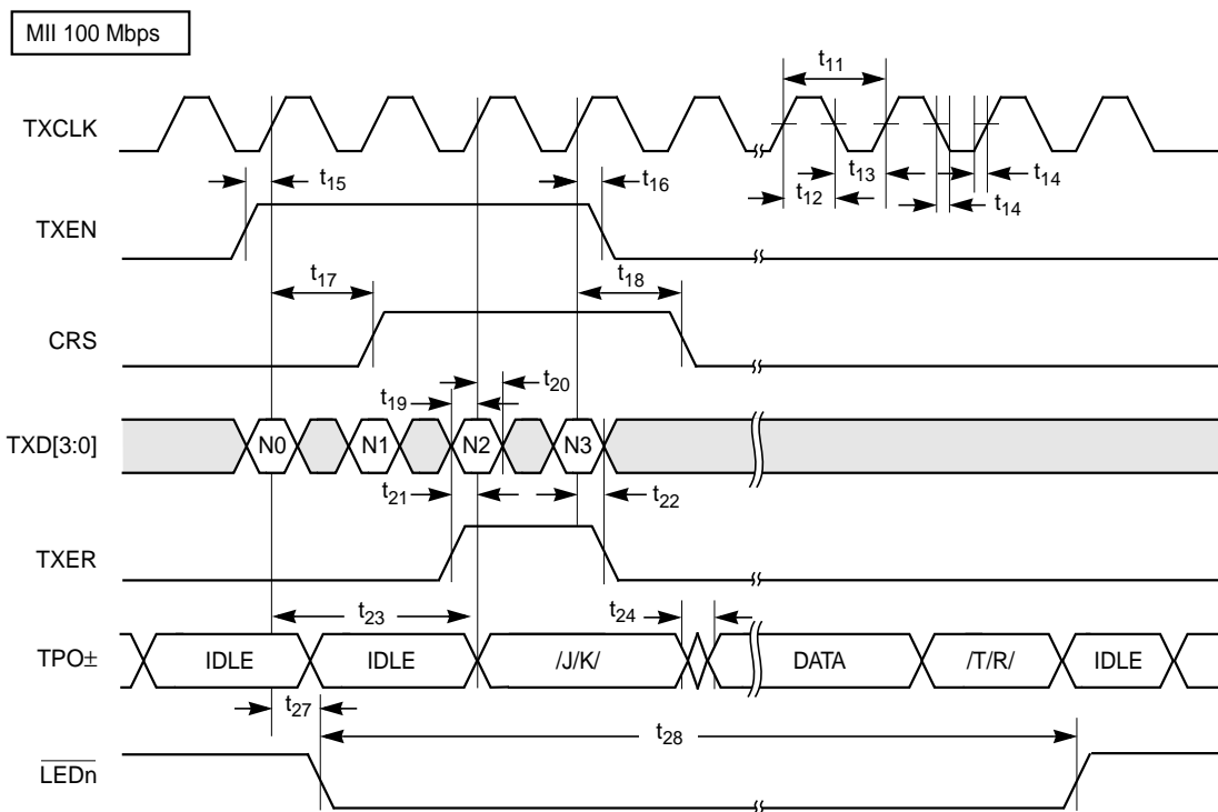
Figure 16 Transmit Timing - 100 Mbps
