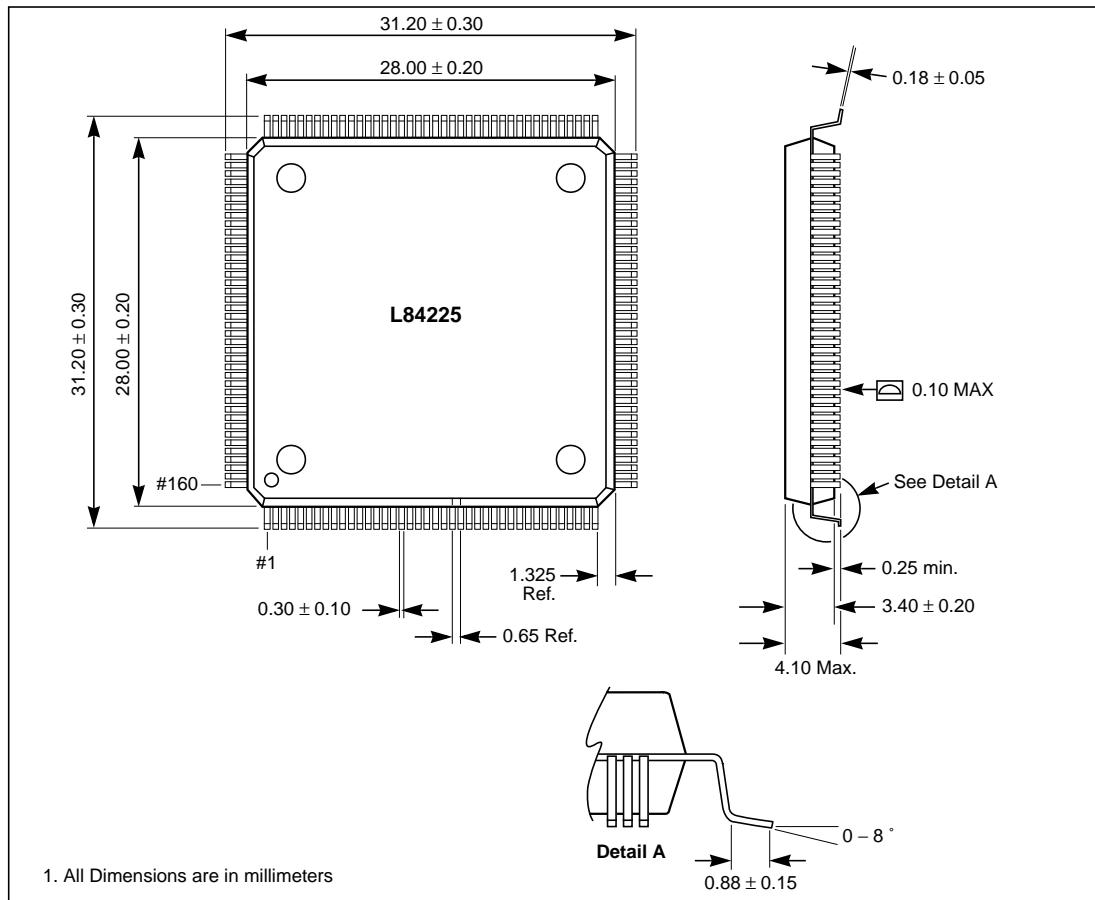
Figure 33 160-Pin PQFP
