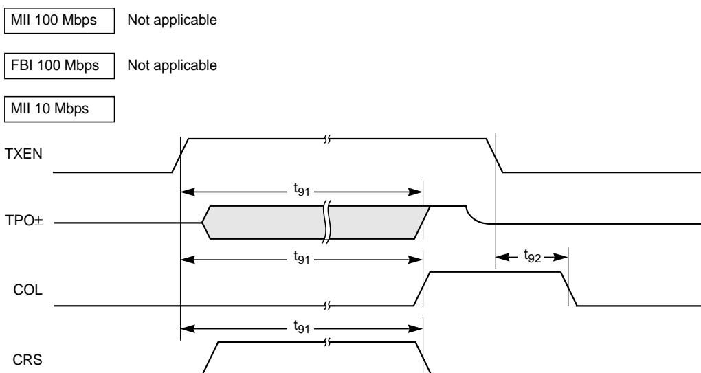
Figure 30 Jabber Timing
