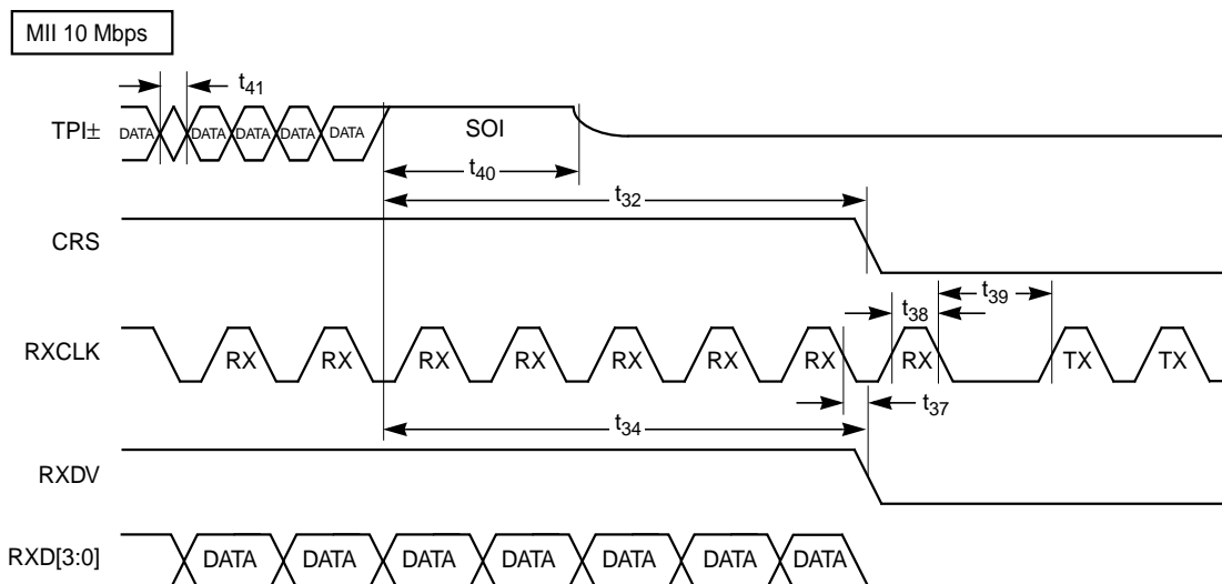
Figure 23 Receive Timing, End of Packet - 10 Mbps, MII
