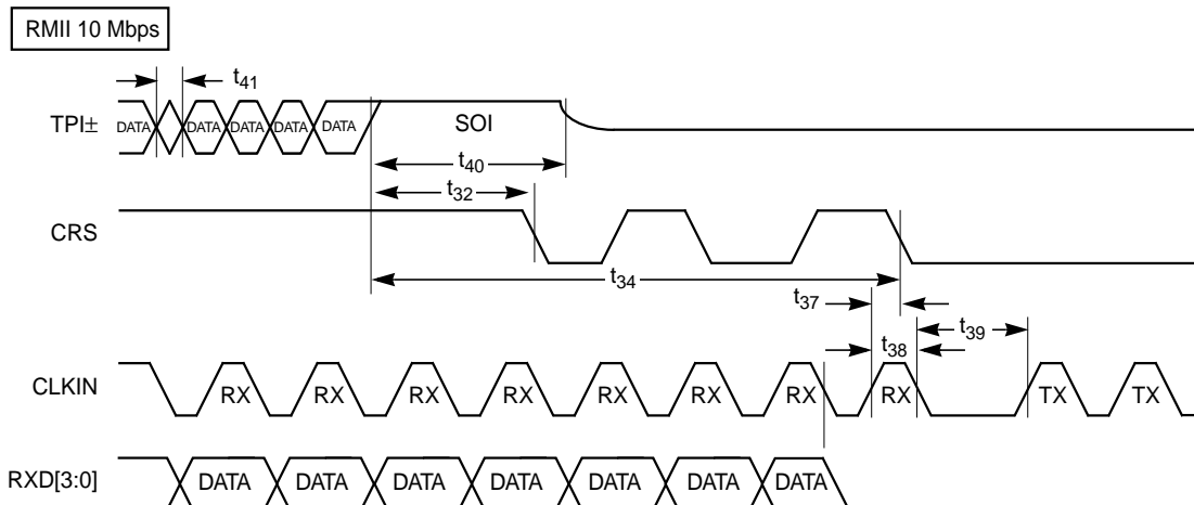
Figure 24 Receive Timing, End of Packet - 10 Mbps, RMII
