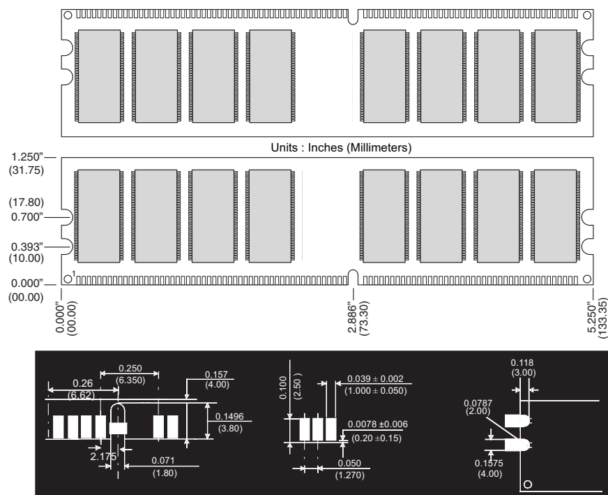
Figure 1: KVR266X64C25/1G 184-Pin DDR SDRAM Module
