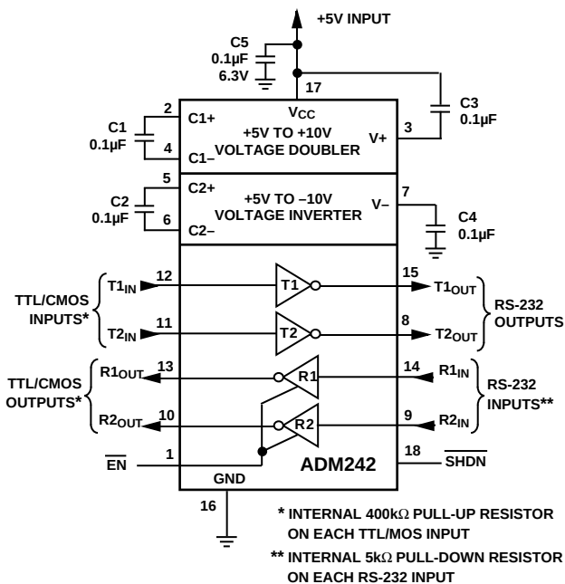
Figure 12. ADM242 Typical Operating Circuit
