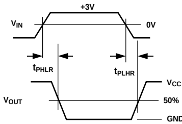
Figure 3. Receiver Propagation Delay Timing
