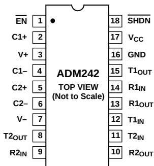
Figure 11. ADM242 DIP/SOIC Pin Configuration
