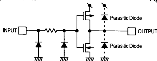
Figure 3. Input Equivalent Circuit
