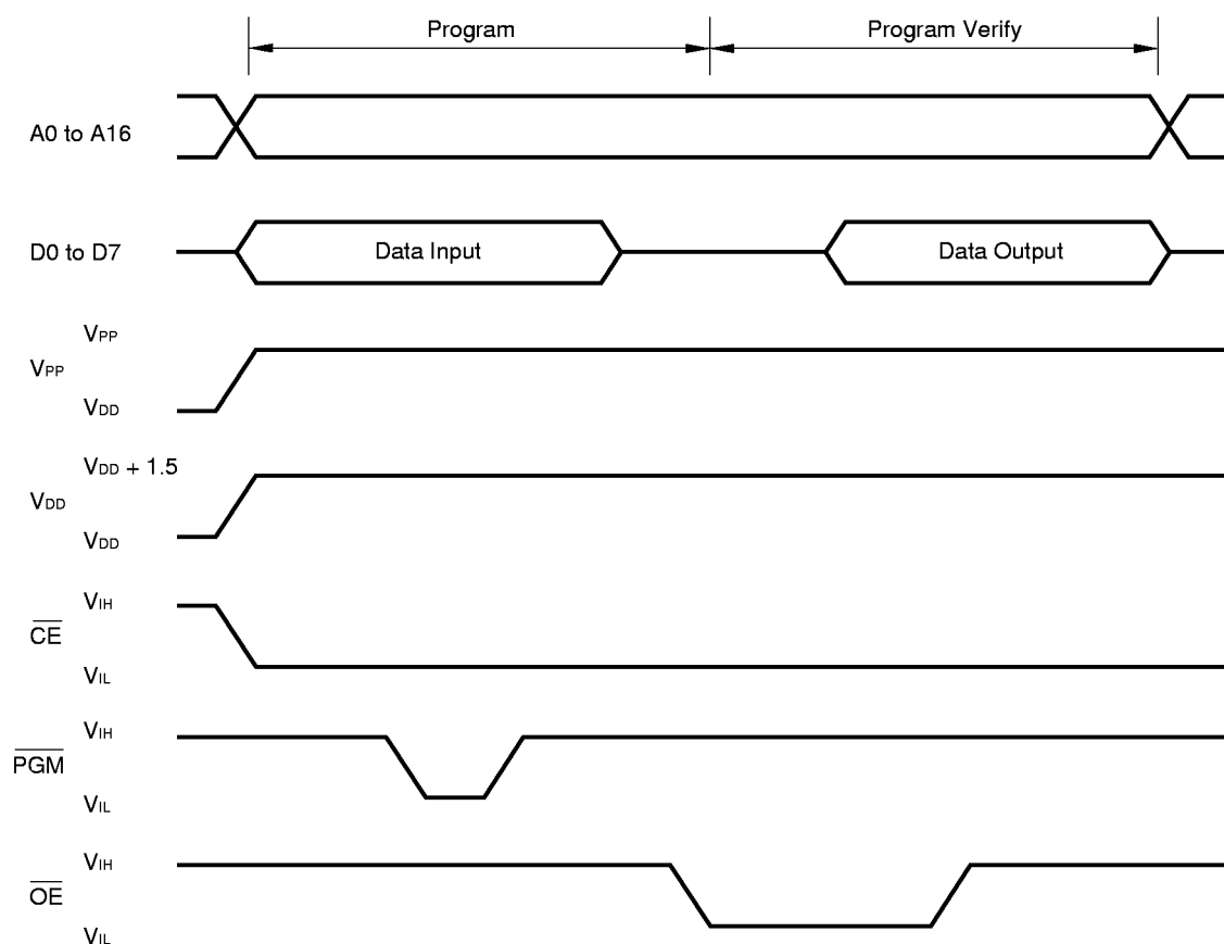
Figure 4-4. Byte Program Mode Timing
