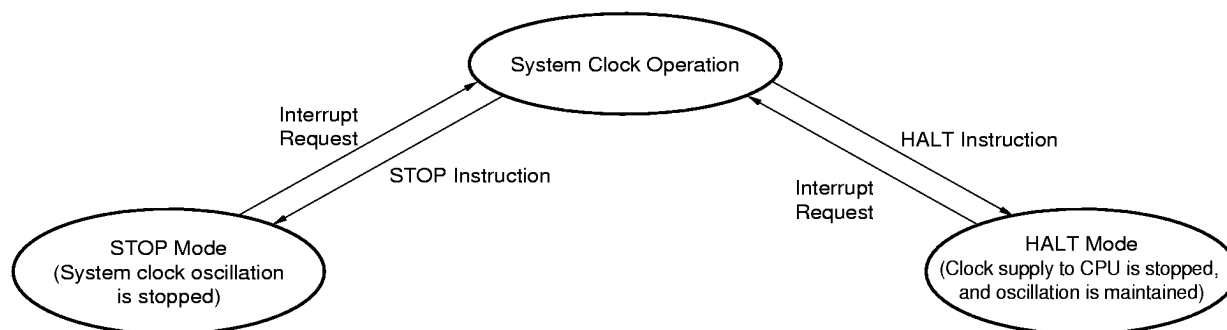
Figure 8-1. Standby Functions
