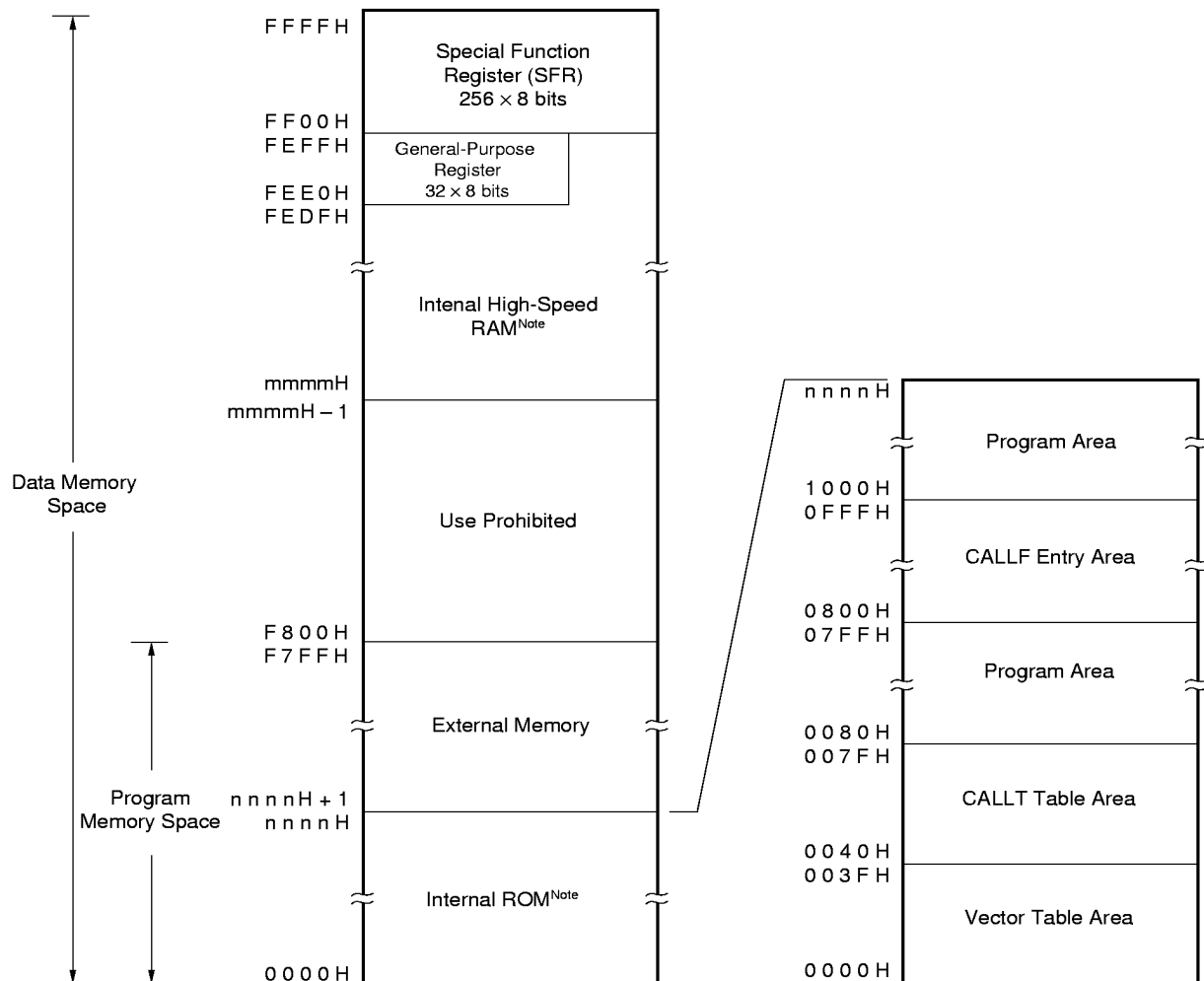
Figure 4-1. Memory Map
