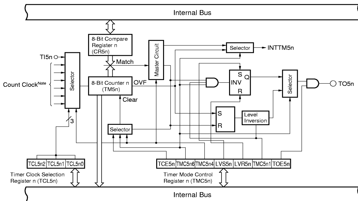
Figure 5-2. 8-Bit Timer/Event Counter Block Diagram
