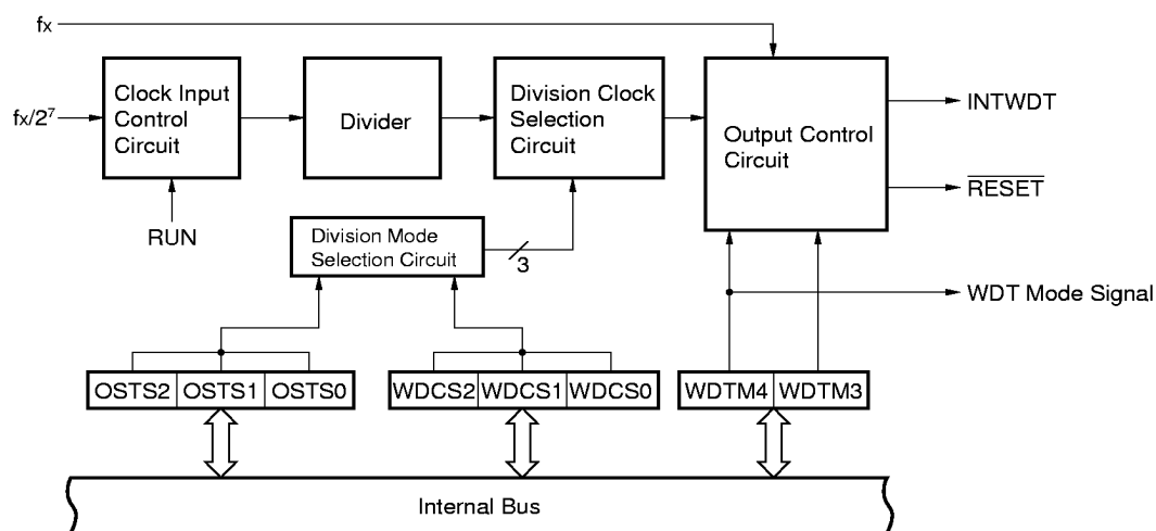
Figure 5-4. Watchdog Timer Block Diagram
