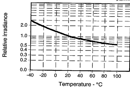
Fig. 2 Threshold Irradiance vs Temperature
