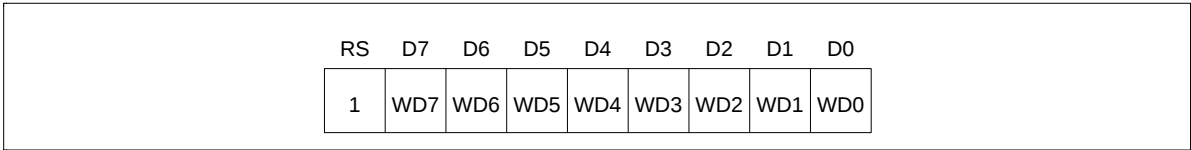
Figure 18 Write Data to RAM Instruction
