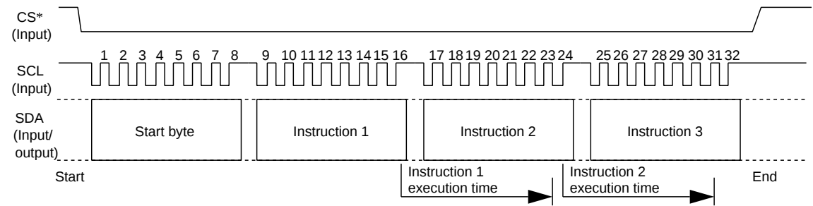
b) Consecutive Data-Transfer Timing Through Clock-Synchronized Serial Bus interface
