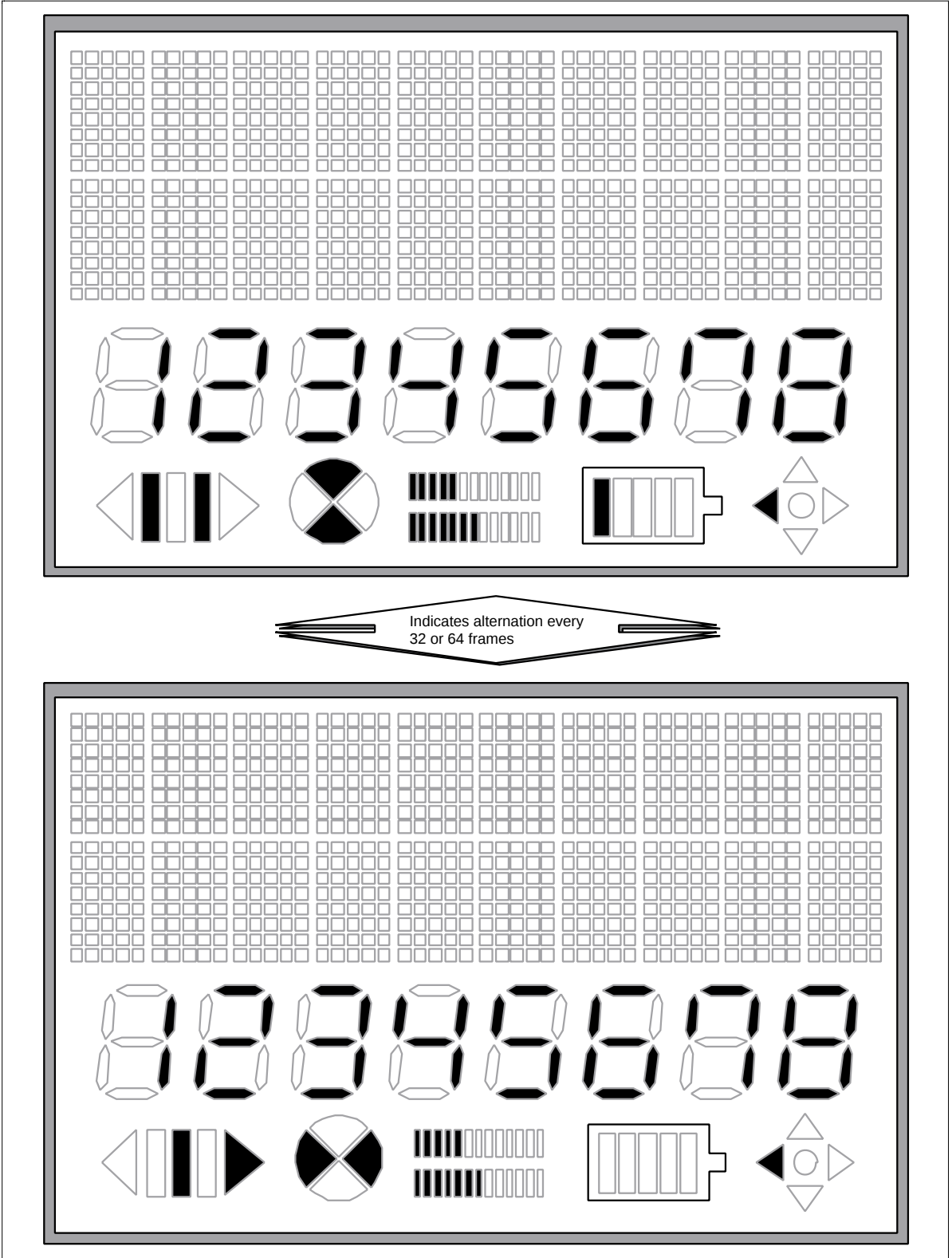
Figure 32 Example of a Segment-Based Display
