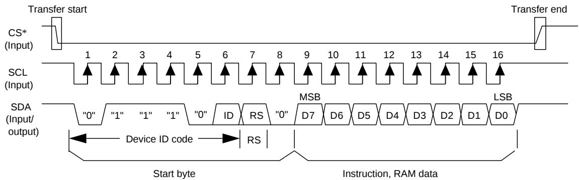
a) Basic Data-Transfer Timing through Clock-Synchronized Serial Bus Interface
