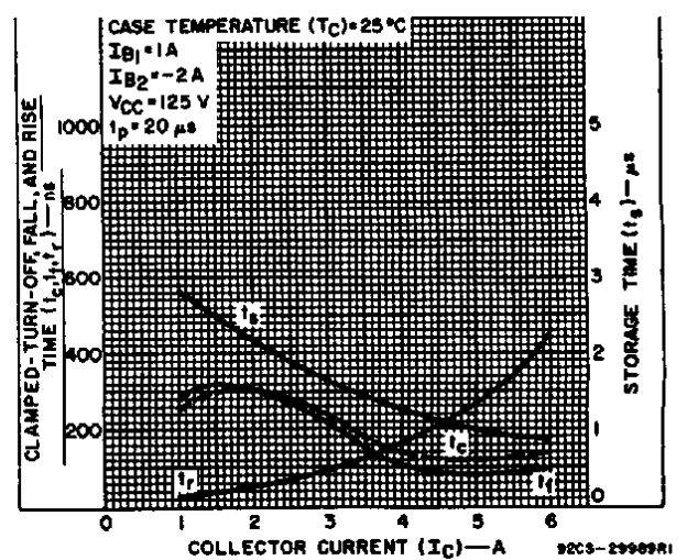
Fig. 11 — Typical saturated-switching-time characteristics for all types.
