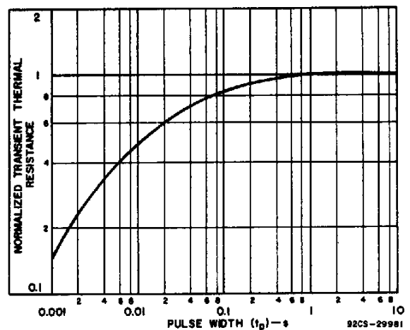
Fig. 2 — Typical thermal-response characteristics for all types.
