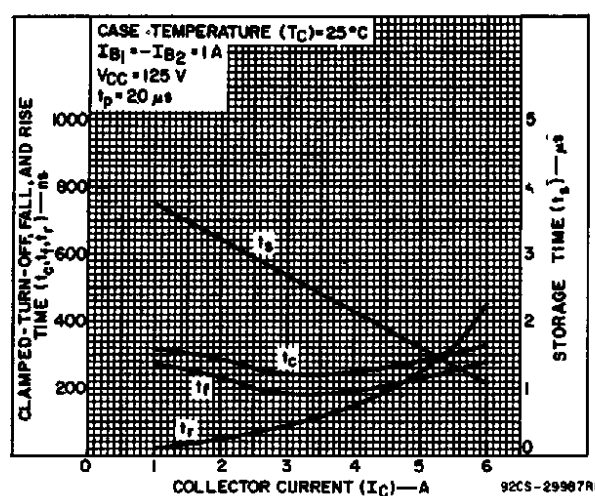
Fig. 9 — Typical saturated-switching-time characteristics for all types.
