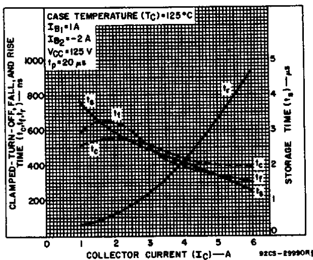
Fig. 12 — Typical saturated-switching-time characteristics for all types.
