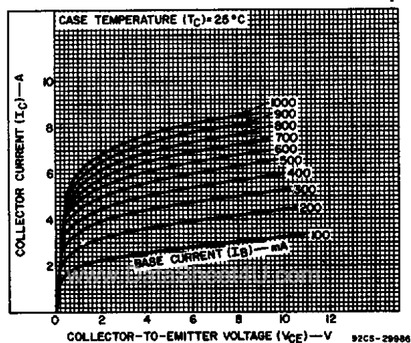
Fig. 8 — Typical output characteristics for all types.
