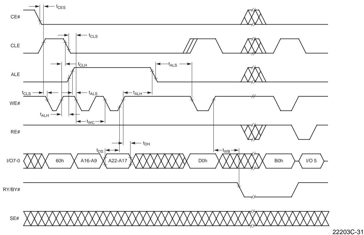
Figure 27. Erase Suspend
