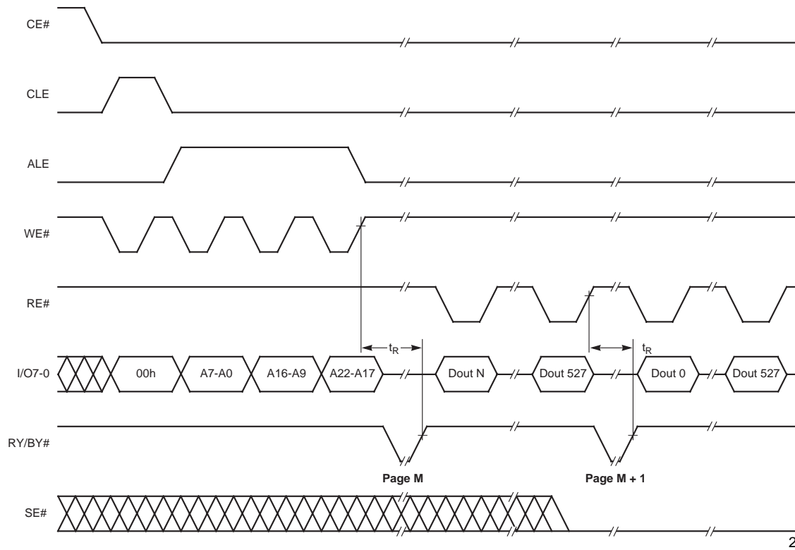
Figure 24. Sequential Read
