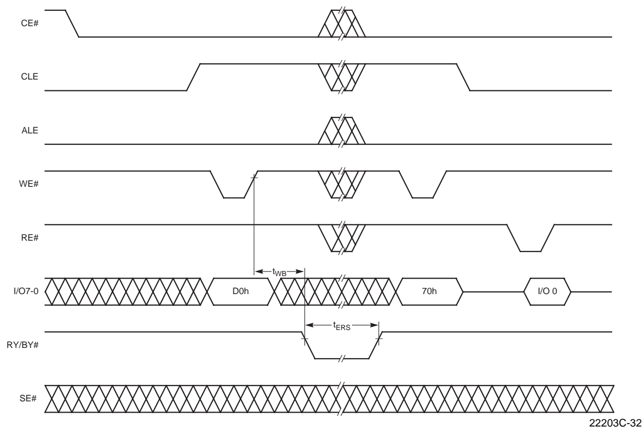
Figure 28. Erase Resume
