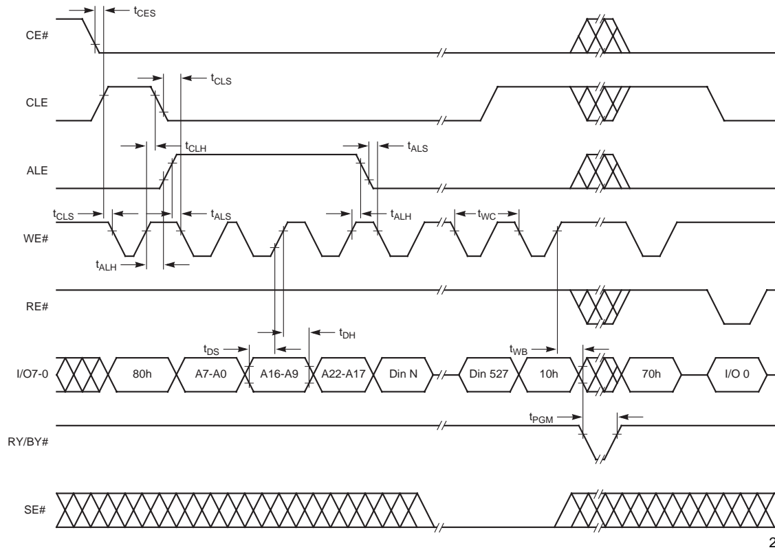
Figure 25. Page Program
