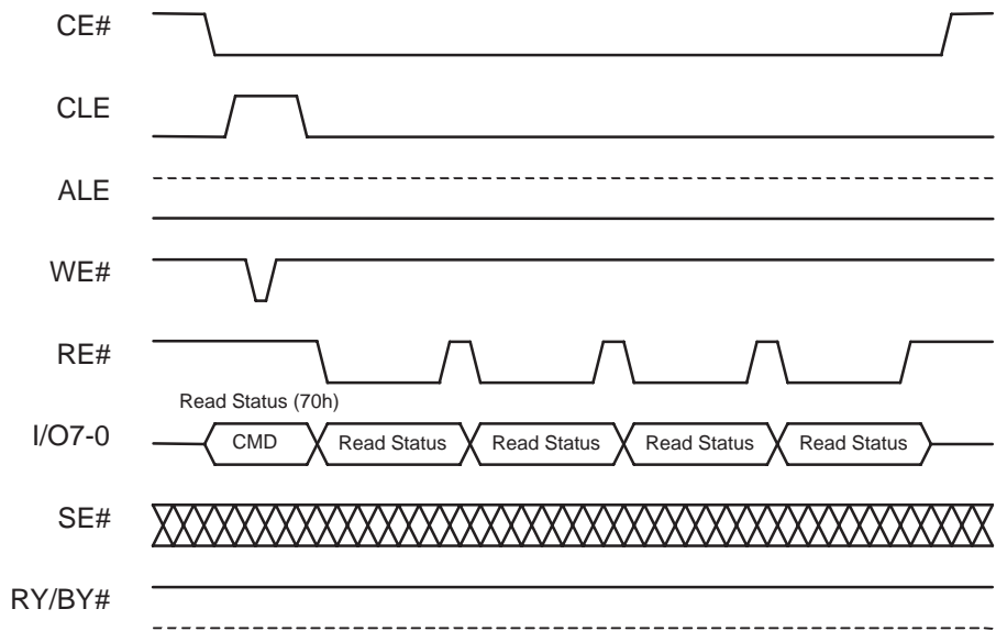
Figure 7. Read Status
