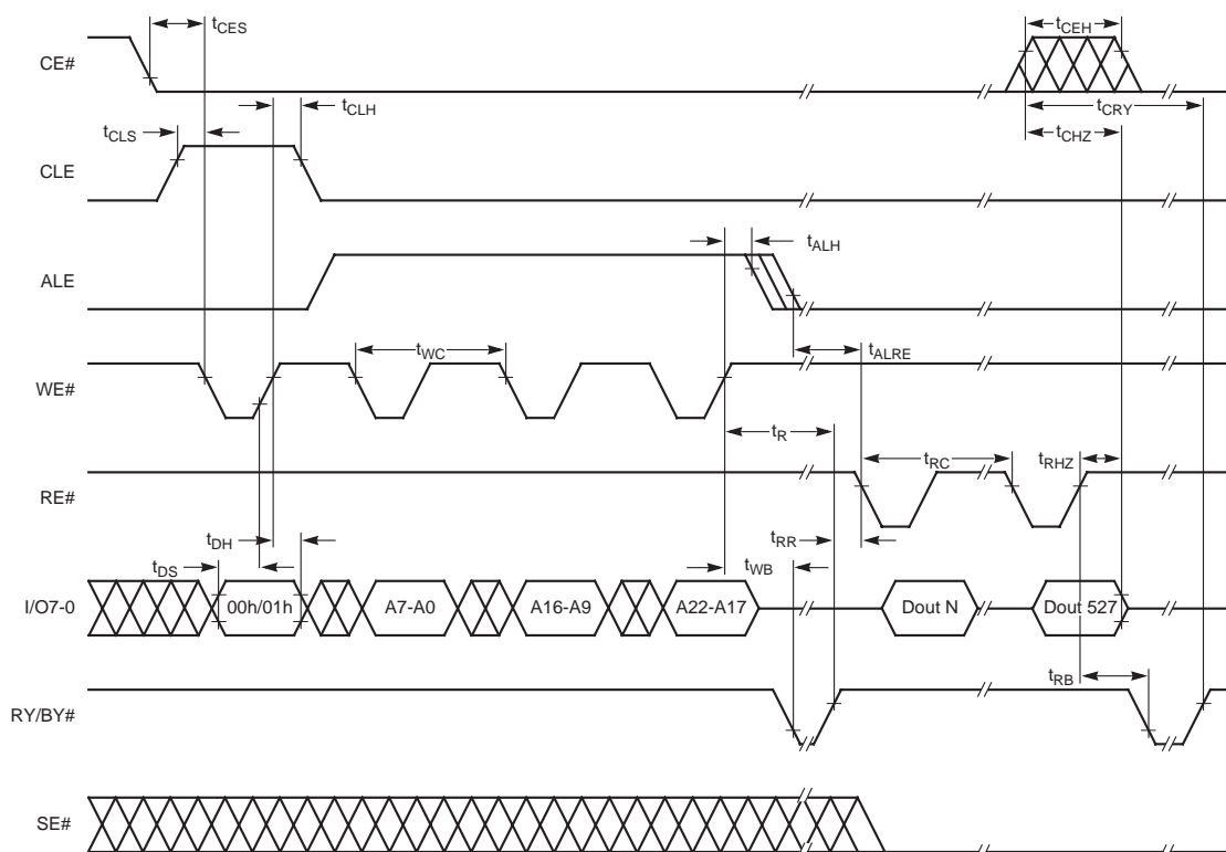
Figure 21. Read Data
