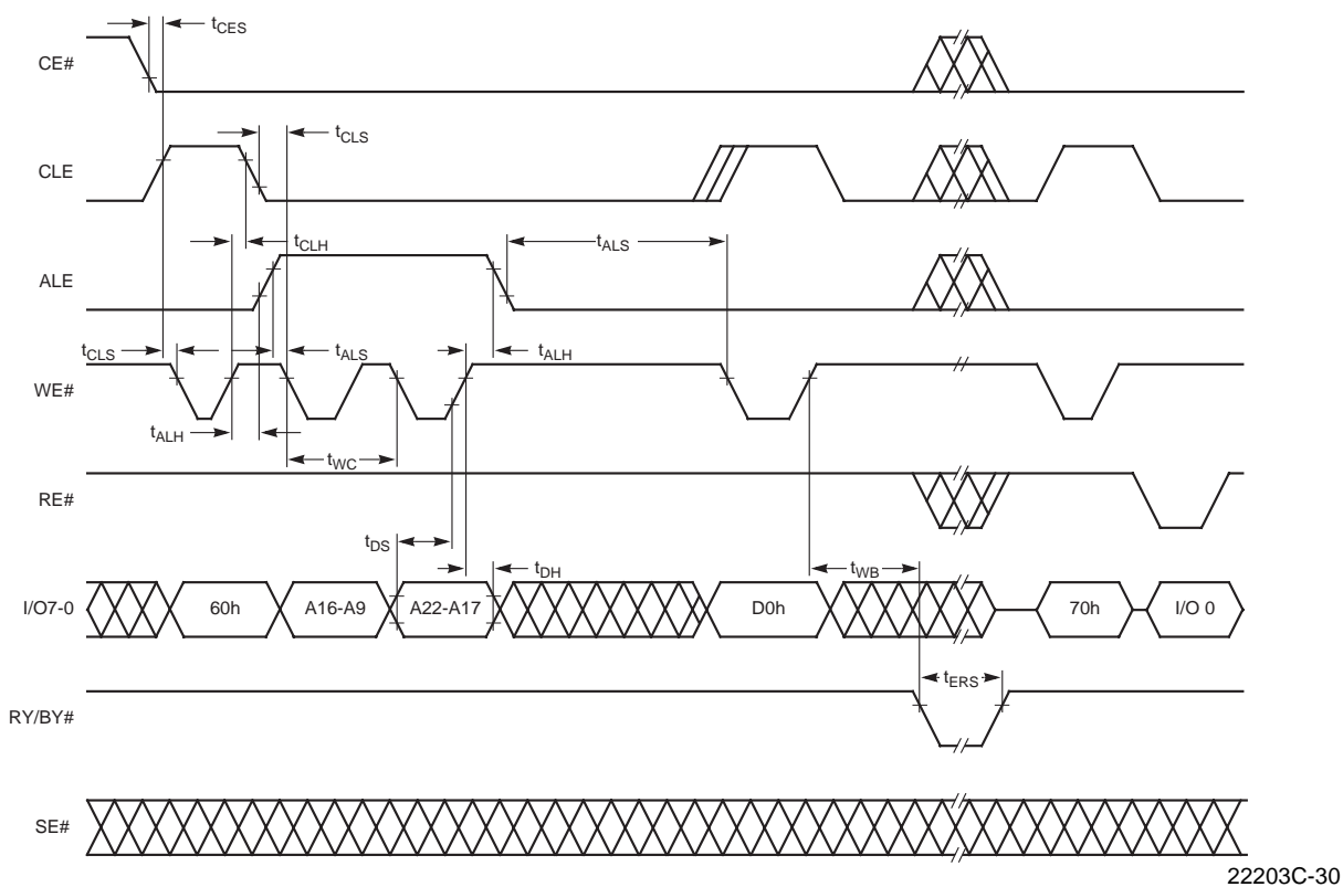
Figure 26. Block Erase
