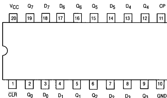
CONNECTION DIAGRAM
