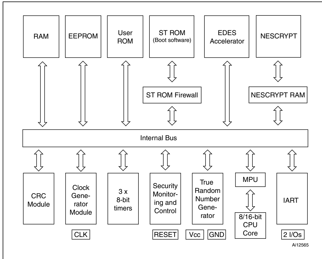
Figure 1. ST23YL80 block diagram
