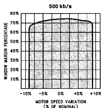
FIGURE 5-2. PC87311A/12 Dynamic Window Margin Performance (Typical performance at V_{CC} = 5.0V , 25^{\circ}C )
