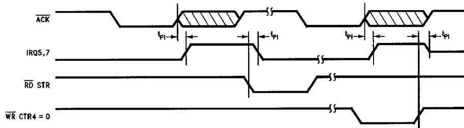
FIGURE 9-15. Parallel Port Interrupt Timing (Extended Mode)
