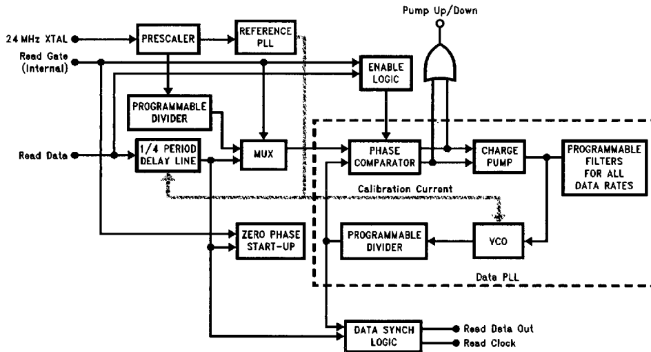
FIGURE 5-1. FDC Data Separator Block Diagram
