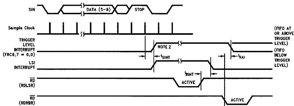
FIGURE 9-6a. Receiver Timing
