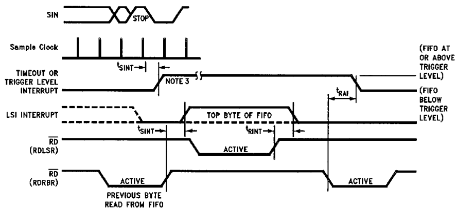
FIGURE 9-6c. PC87312 Timeout Receiver Timing
