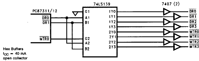
FIGURE 10-1. PC87311A/12 Four Floppy Drive Circuit
