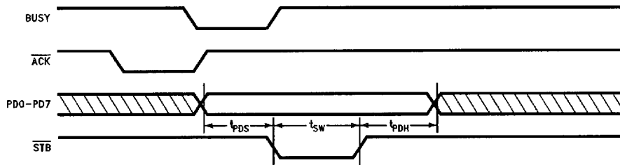
FIGURE 9-16. Typical Parallel Port Data Exchange
