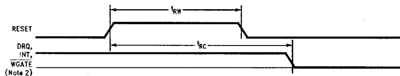
FIGURE 9-9. Reset Timing
