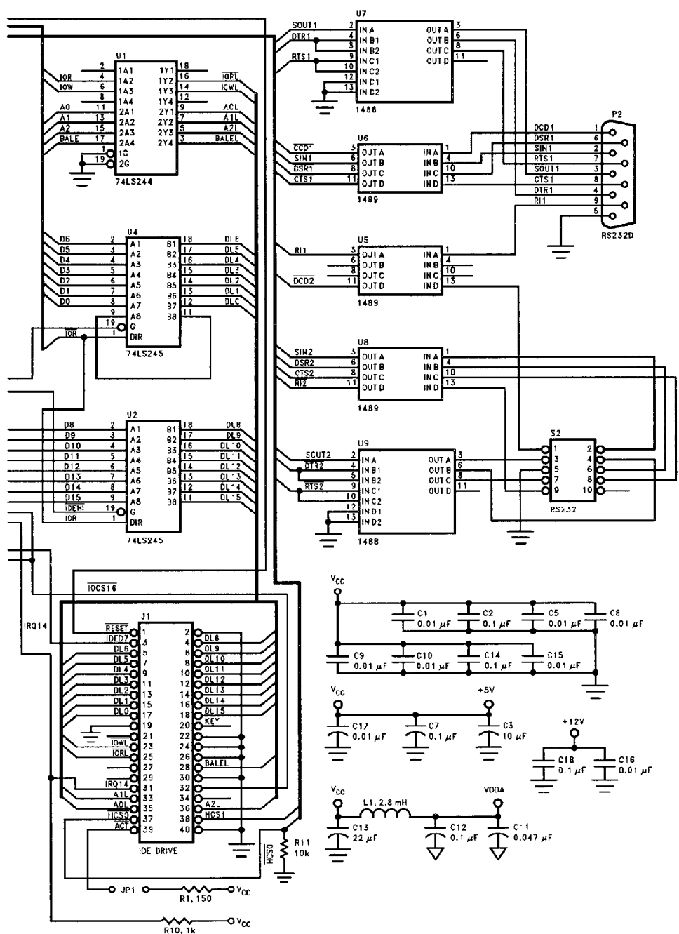
FIGURE 10-3. PC87311A/12 Adapter Card Schematic (Continued)
