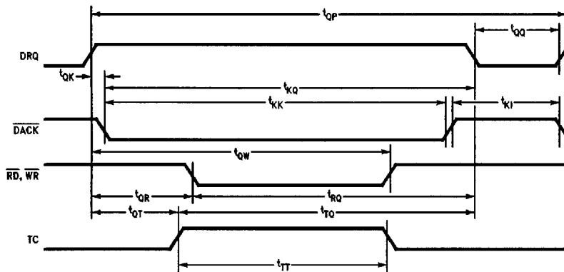
FIGURE 9-8. DMA Timing
