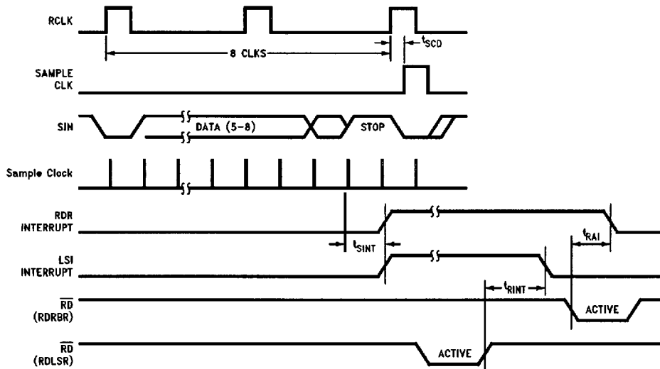
FIGURE 9-6a. Receiver Timing
