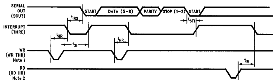
FIGURE 9-5. Transmitter Timing
