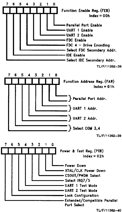
FIGURE 2-1. PC87311A/12 Configuration Registers
