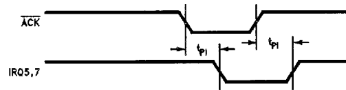
FIGURE 9-14. Parallel Port Interrupt Timing (Compatible Mode)
