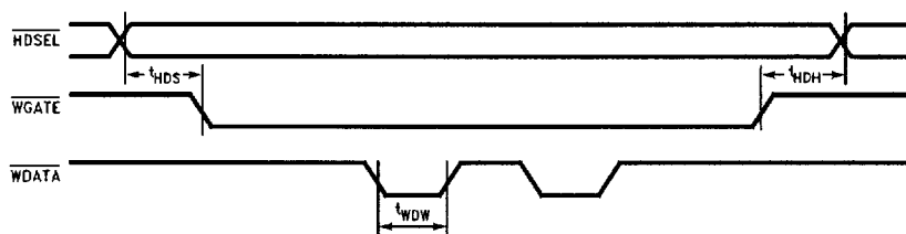
FIGURE 9-10. Write Data Timing
