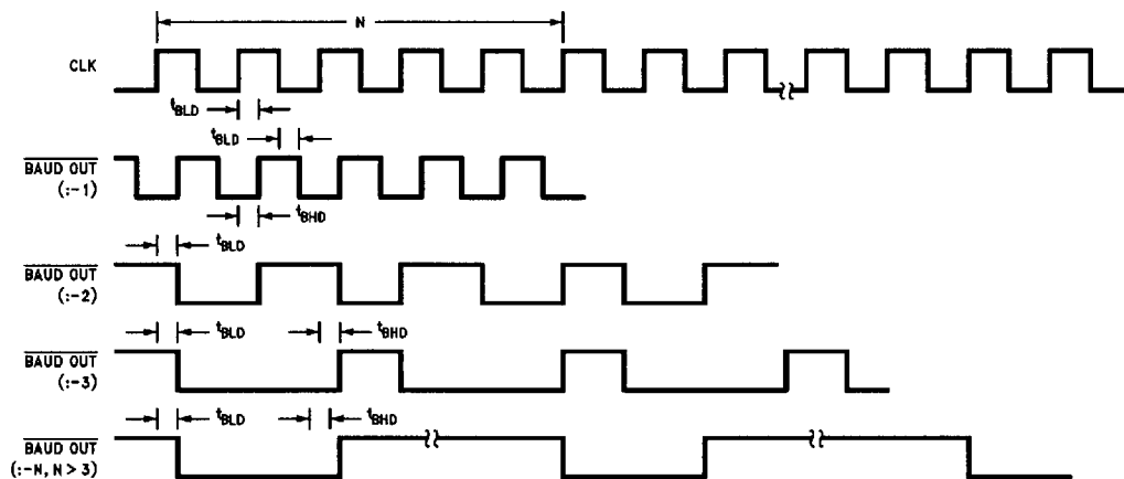
FIGURE 9-4. Baudout Timing
