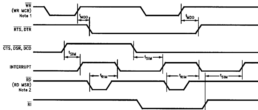
FIGURE 9-7. MODEM Control Timing
