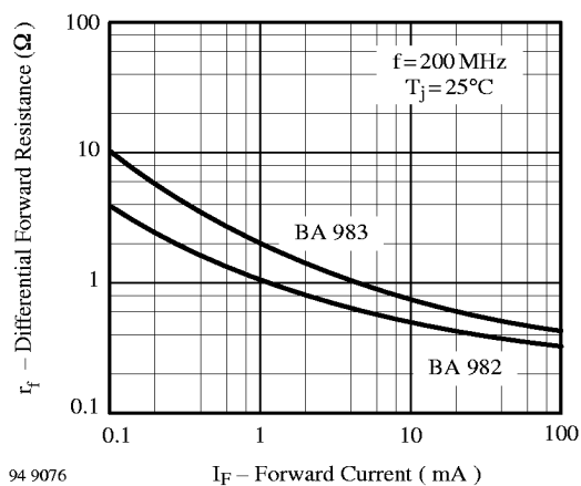
Figure 1. Differential Forward Resistance vs. Forward Current
