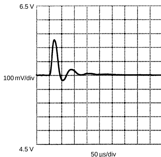
Figure 8 Load Step Response Load Step 6.0 A to 3.0 A (Full Load to Half Load)
