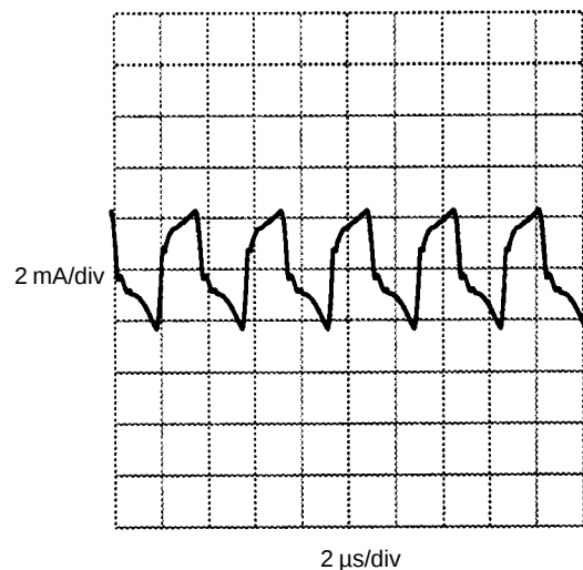
Figure 2 Input Ripple Voltage V_{IN} = 28\text{ V}_{DC} , Full Load
