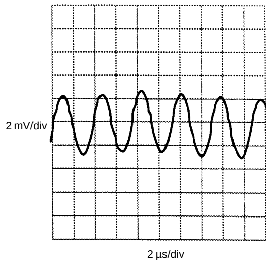
Figure 1 Output Ripple Voltage V_{IN} = 28\text{ V}_{DC} , Full Load
