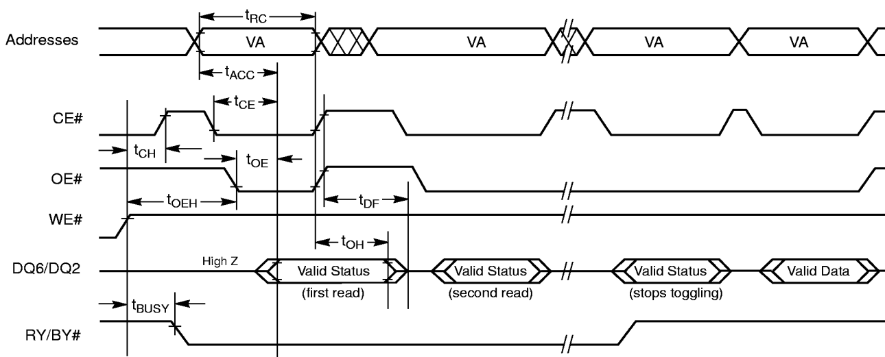
Figure 16. Data# Polling Timings (During Embedded Algorithms)
