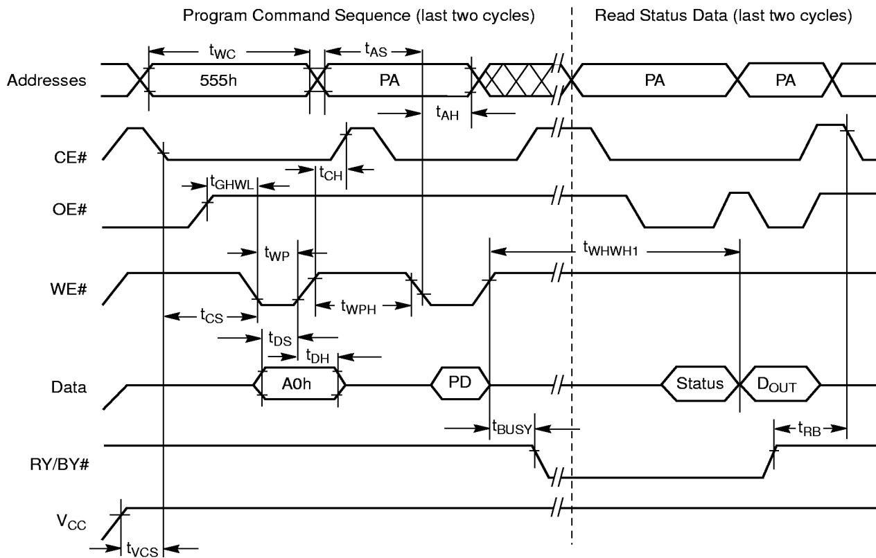
Figure 14. Program Operation Timings
