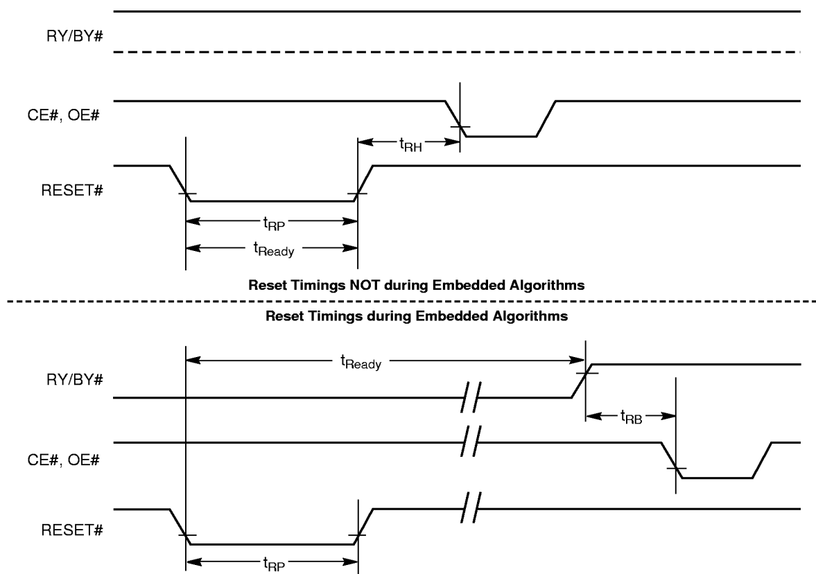
Figure 13. RESET# Timings
