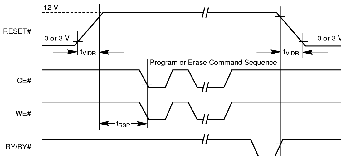
Figure 19. Temporary Sector Unprotect Timing Diagram
