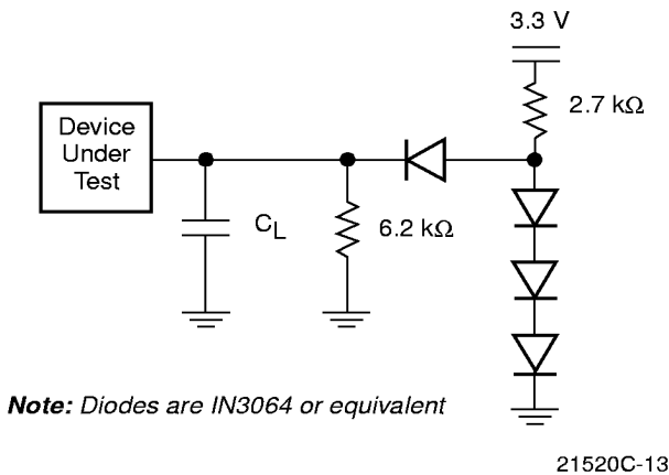
Figure 10. Test Setup
