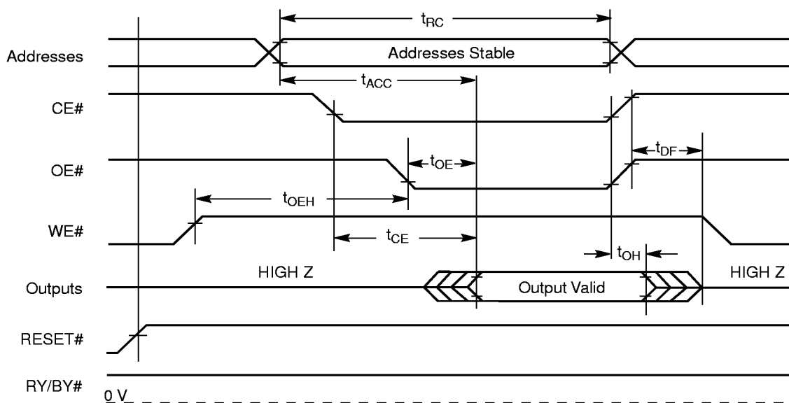
Figure 12. Read Operations Timings
