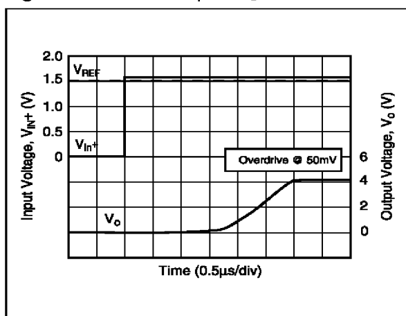
Figure 3 : Transition speed @ 50mV overdrive
