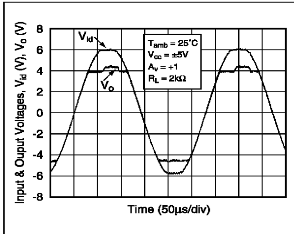
Figure 5 : Behaviour with TSH22
