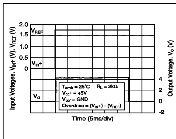
Figure 4 : Transition speed @ 250mV overdrive
