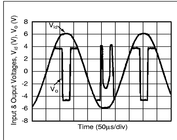
Figure 6 : Saturation behaviour with 15MHz standard operational amplifier
