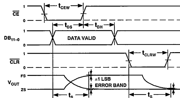
Figure 2. Timing Diagram
