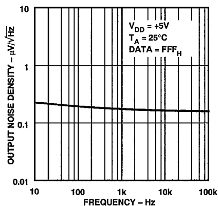
Figure 20. Output Voltage Noise Density vs. Frequency
