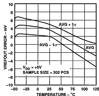
Figure 25. Reference Error vs. Temperature
