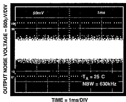
Figure 8. Broadband Noise
