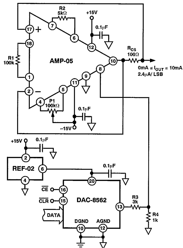
Figure 38. A High-Compliance, Digitally Controlled Precision Current Source
