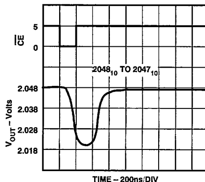
Figure 12. Midscale Transition Performance
