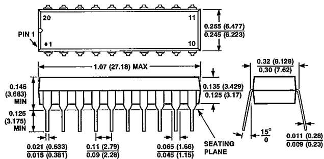
20-Pin Plastic DIP (P-Suffix)
