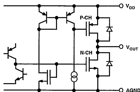
Figure 4. Equivalent Analog Output Circuit
