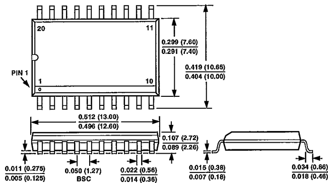
20-Lead SOIC (S-Suffix)
