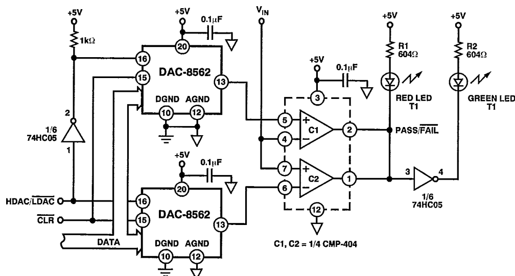
Figure 39. A Digitally Programmable Window Detector
