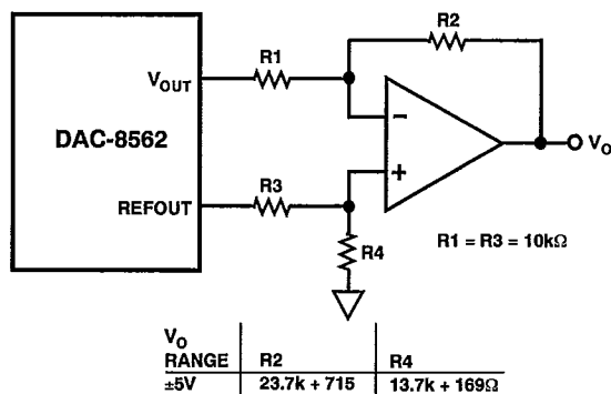
Figure 35. Bipolar Output Operation Without Trim Version 2
