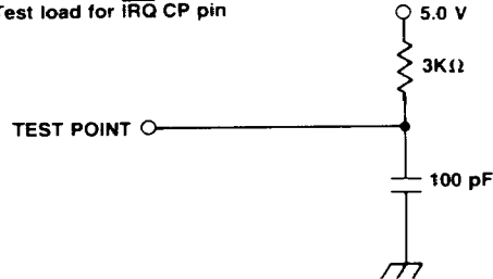
Test load for \overline{IRQ} CP pin
