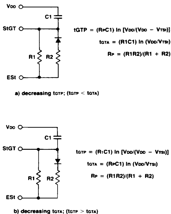
Figure 4. Guard Time Adjustment
