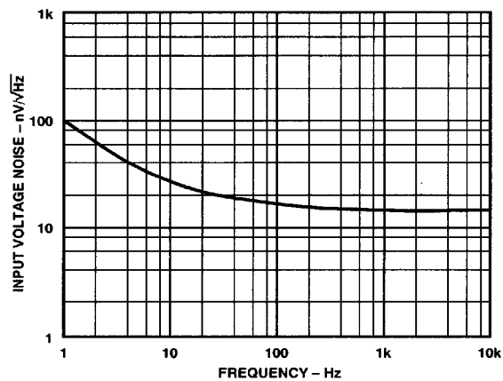
Figure 11. Input Voltage Noise vs. Frequency
