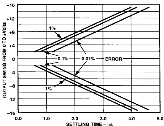
Figure 15. Output Swing and Error vs. Settling Time
