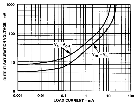
Figure 18. Output Saturation Voltage vs. Load Current
