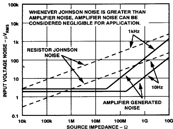
Figure 40. Total Noise vs. Source Impedance
