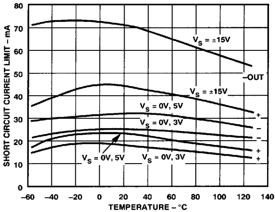
Figure 20. Short Circuit Current Limit vs. Temperature
