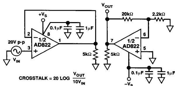
Figure 28. Crosstalk Test Circuit
