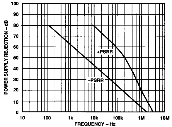
Figure 22. Power Supply Rejection vs. Frequency
