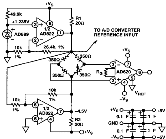
Figure 47. Low Dropout Bipolar Bridge Driver
