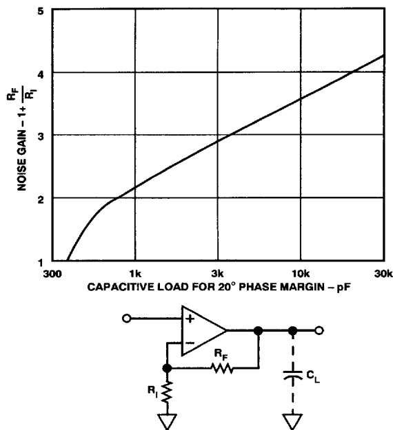
Figure 42. Capacitive Load Tolerance vs. Noise Gain
