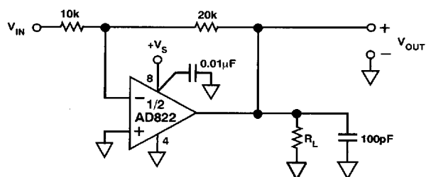
Figure 33. Gain of Two Inverter
