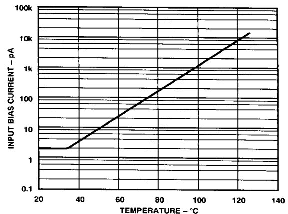
Figure 6. Input Bias Current vs. Temperature; V_S = 5\text{ V} , V_{CM} = 0
