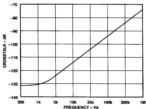
Figure 25. Crosstalk vs. Frequency
