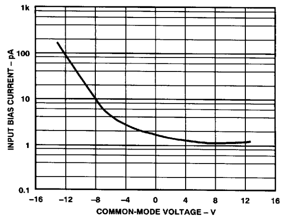
Figure 5. Input Bias Current vs. Common-Mode Voltage; V_S = \pm 15\text{ V}
