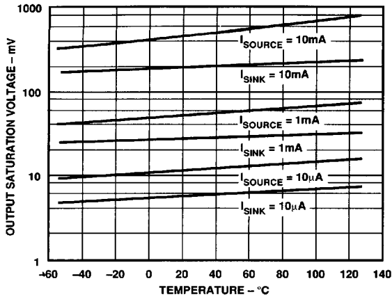
Figure 19. Output Saturation Voltage vs. Temperature
