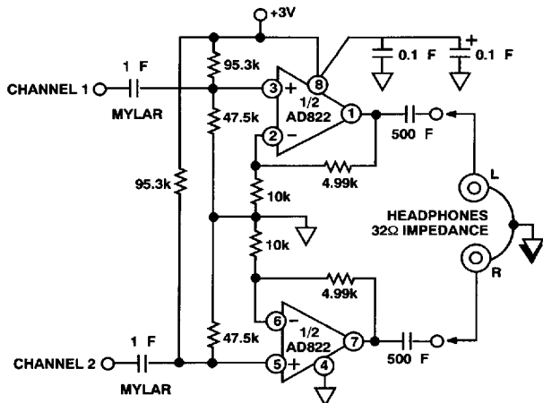
Figure 46. 3 Volt Single Supply Stereo Headphone Driver
