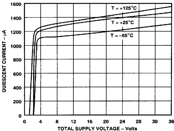
Figure 21. Quiescent Current vs. Supply Voltage vs. Temperature
