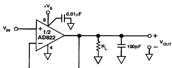
Figure 32. Unity-Gain Follower
