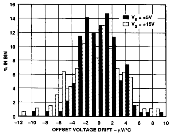
Figure 2. Typical Distribution of Offset Voltage Drift (100 Units)
