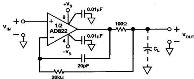
Figure 43. Extending Unity Gain Follower Capacitive Load Capability Beyond 350 \text{ pF}
