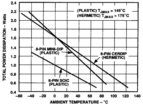
Figure 24. Maximum Power Dissipation vs. Temperature for Plastic and Hermetic Packages
