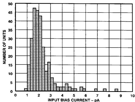
Figure 3. Typical Distribution of Input Bias Current (213 Units)
