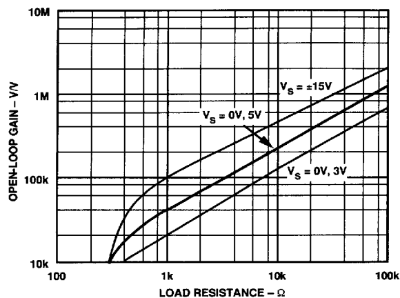
Figure 7. Open-Loop Gain vs. Load Resistance
