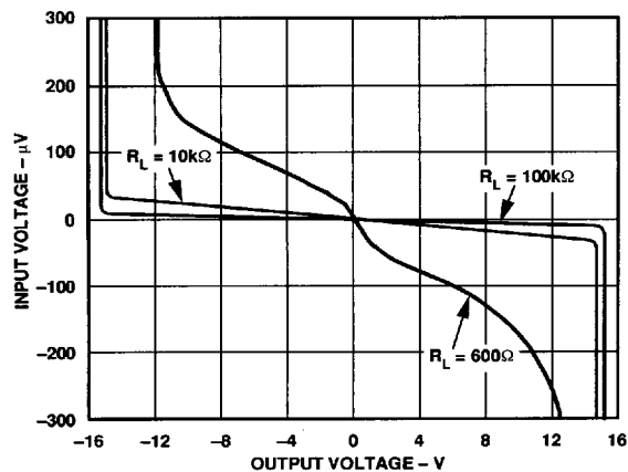
Figure 9. Input Error Voltage vs. Output Voltage for Resistive Loads
