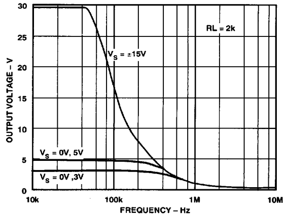
Figure 23. Large Signal Frequency Response
