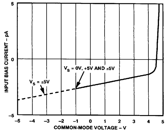
Figure 4. Input Bias Current vs. Common-Mode Voltage; V_S = +5\text{ V} , 0\text{ V} and V_S = \pm 5\text{ V}
