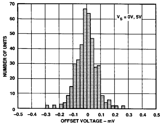
Figure 1. Typical Distribution of Offset Voltage (390 Units)
