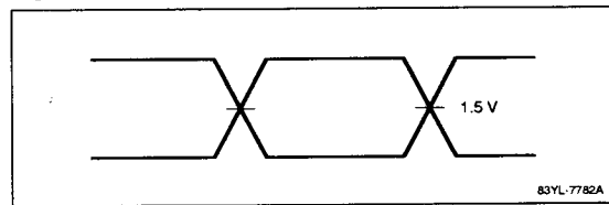
Figure 2. Output Timing
