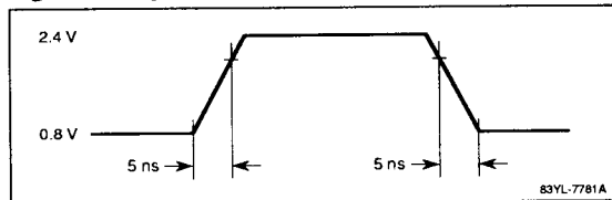
Figure 1. Input Timing
