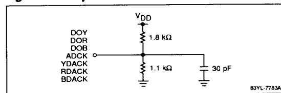
Figure 3. Output Load
