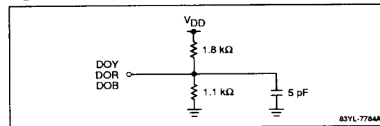
Figure 4. Output Load ( t_{LZ} and t_{HZ} )
