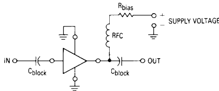
Figure 11. Typical Biasing Configuration
