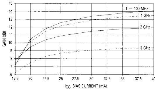
Figure 9. Gain versus Bias Current
