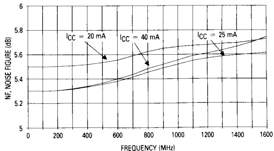
Figure 2. Noise Figure versus Frequency
