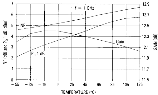
Figure 10. Output Power at 1 dB Gain Compression Noise Figure and Gain versus Temperature
