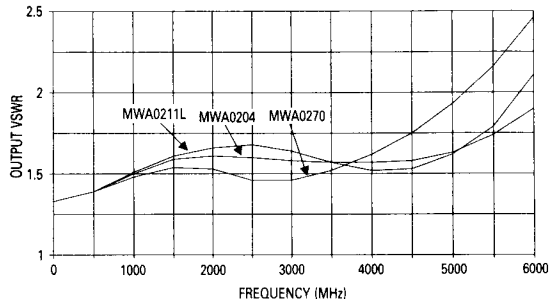
Figure 4. Output VSWR versus Frequency
