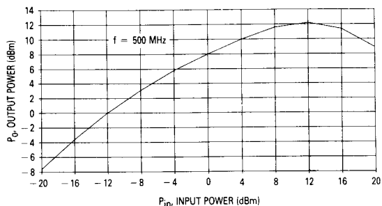
Figure 6. Output Power versus Power
