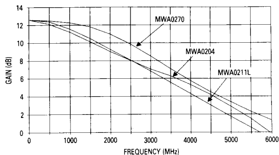
Figure 1. Gain versus Frequency
