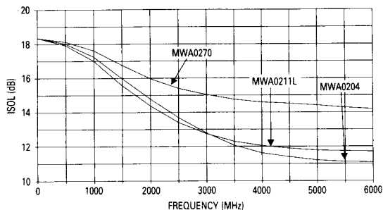
Figure 5. Reverse Isolation versus Frequency
