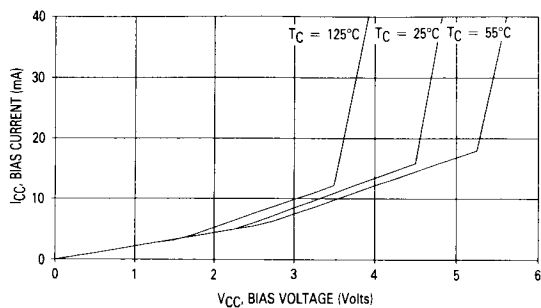
Figure 7. Bias Current versus Bias Voltage
