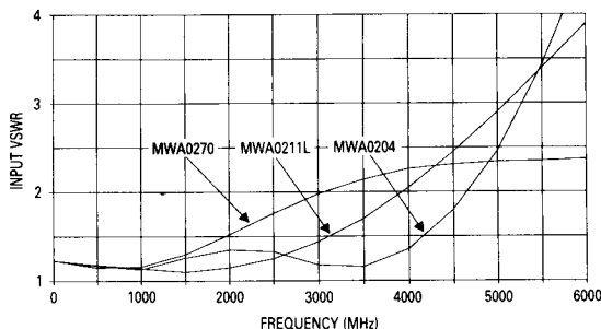
Figure 3. Input VSWR versus Frequency
