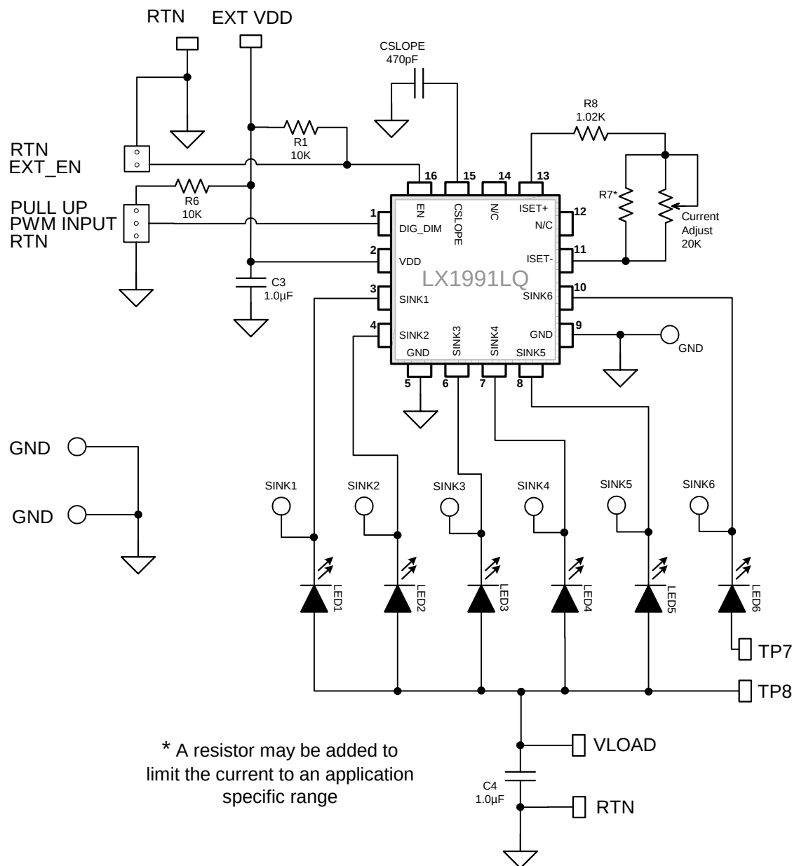
Figure 2 – Schematic
