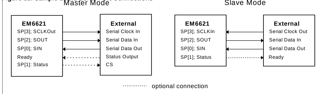
Figure 18. Sample Basic Serial Port Connections
