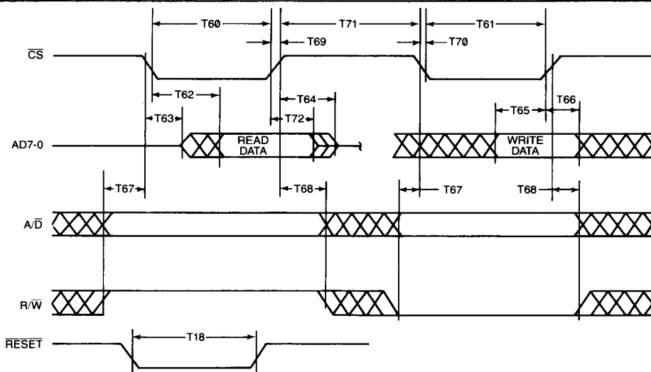
FIGURE 22—SYSTEM BUS PERIPHERAL TIMING
