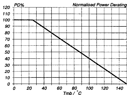
Fig. 1. Normalised power derating. PD\% = 100 \cdot P_D / P_{D 25^\circ\text{C}} = f(T_{mb})
