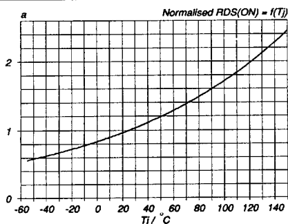
Fig. 9. Normalised drain-source on-state resistance. a = R_{DS(ON)}/R_{DS(ON)25^\circ\text{C}} = f(T_J) ; I_D = 6.5 \text{ A} ; V_{GS} = 10 \text{ V}
