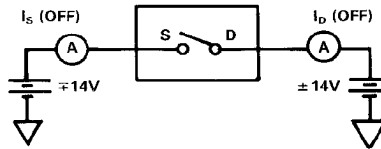
Test Circuit 2
