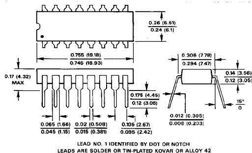
16-Pin Plastic (N-16)
