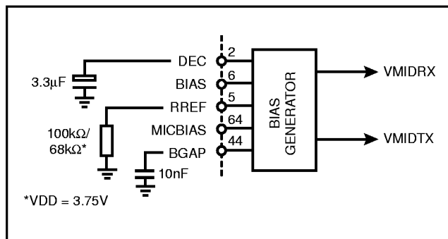
Fig. 16 Bias Circuits
