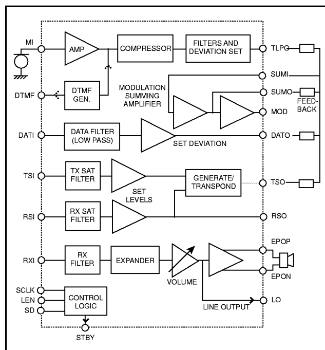
Fig. 2 ACE9040 Simplified Block Diagram
