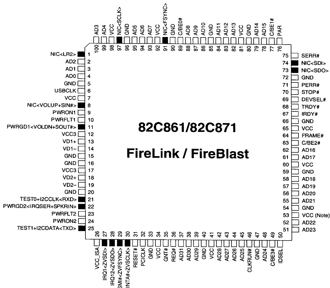
Figure 3-1 LQFP Pin Diagram (Note)
