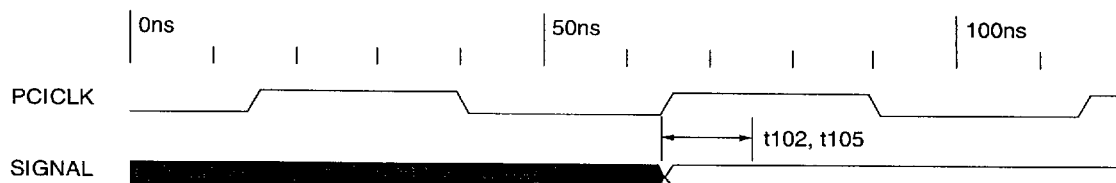
Figure 6-3 Output Delay Timing Waveform
