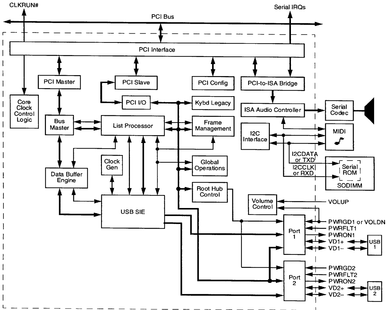
Figure 2-4 FireBlast Block Diagram
