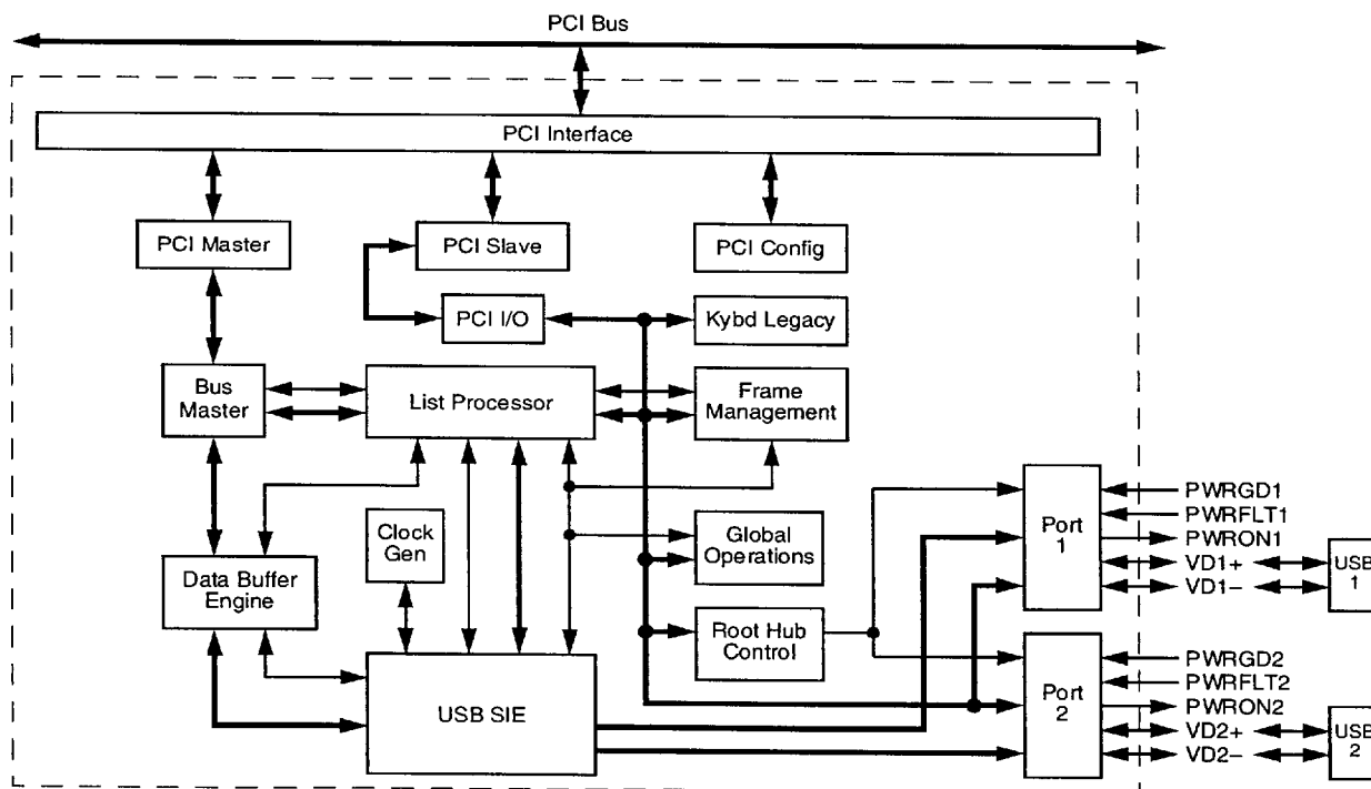
Figure 2-1 FireLink "CMD-based" Type Block Diagram
