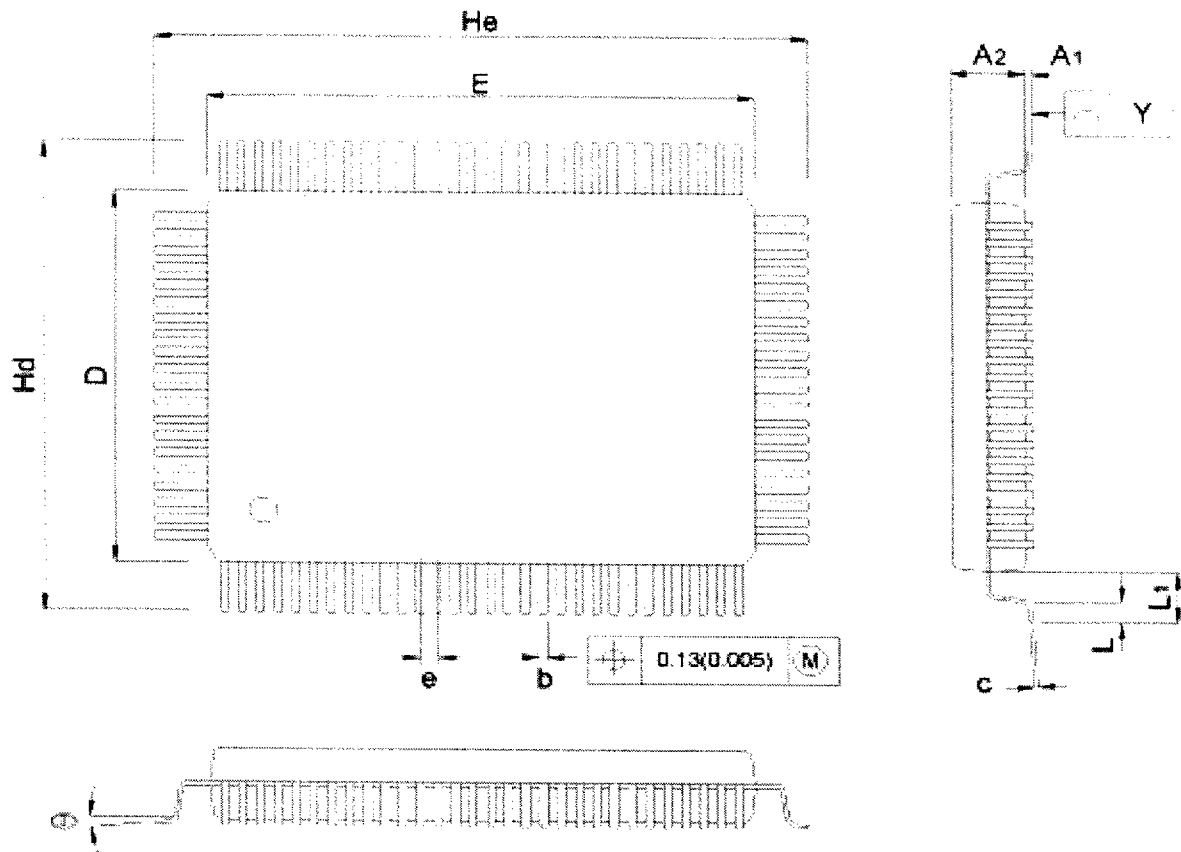
Figure 7-2 100-Pin Quad Flat Pack (QFP)
