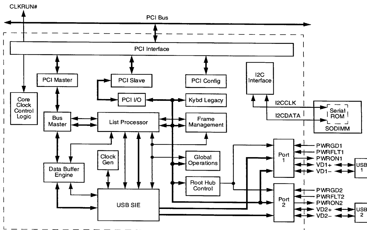
Figure 4-1 USB Functional Block Diagram
