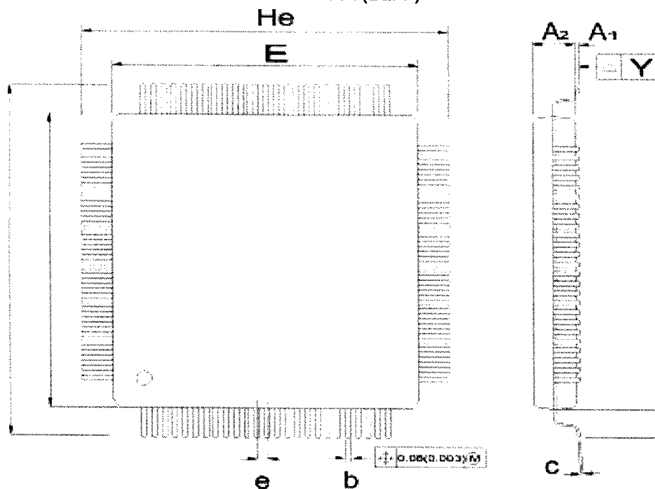
Figure 7-1 100-Pin Low-Profile Quad Flat Pack (LQFP)
