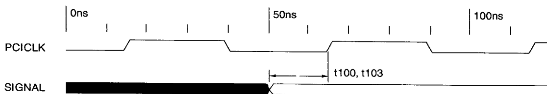
Figure 6-1 Setup Timing Waveform
