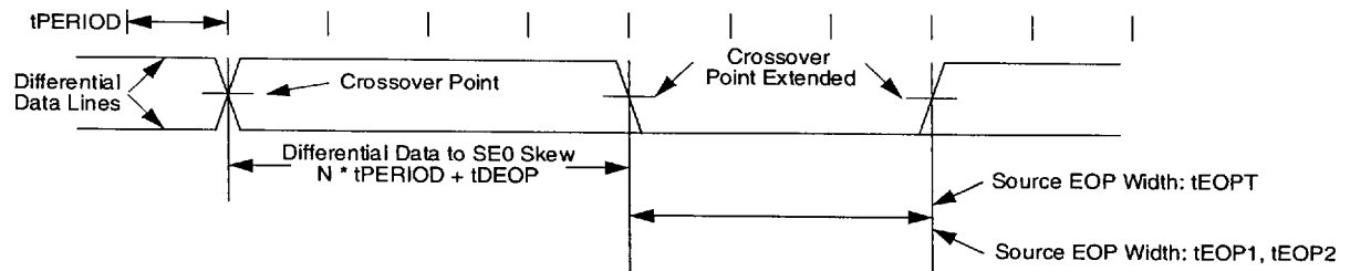
Figure 6-5 Differential to EOP Transition Skew and EOP Width
