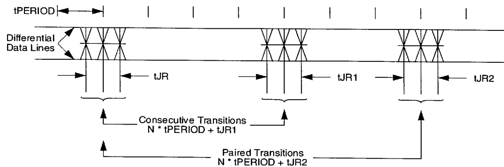
Figure 6-6 Receiver Jitter Tolerance
