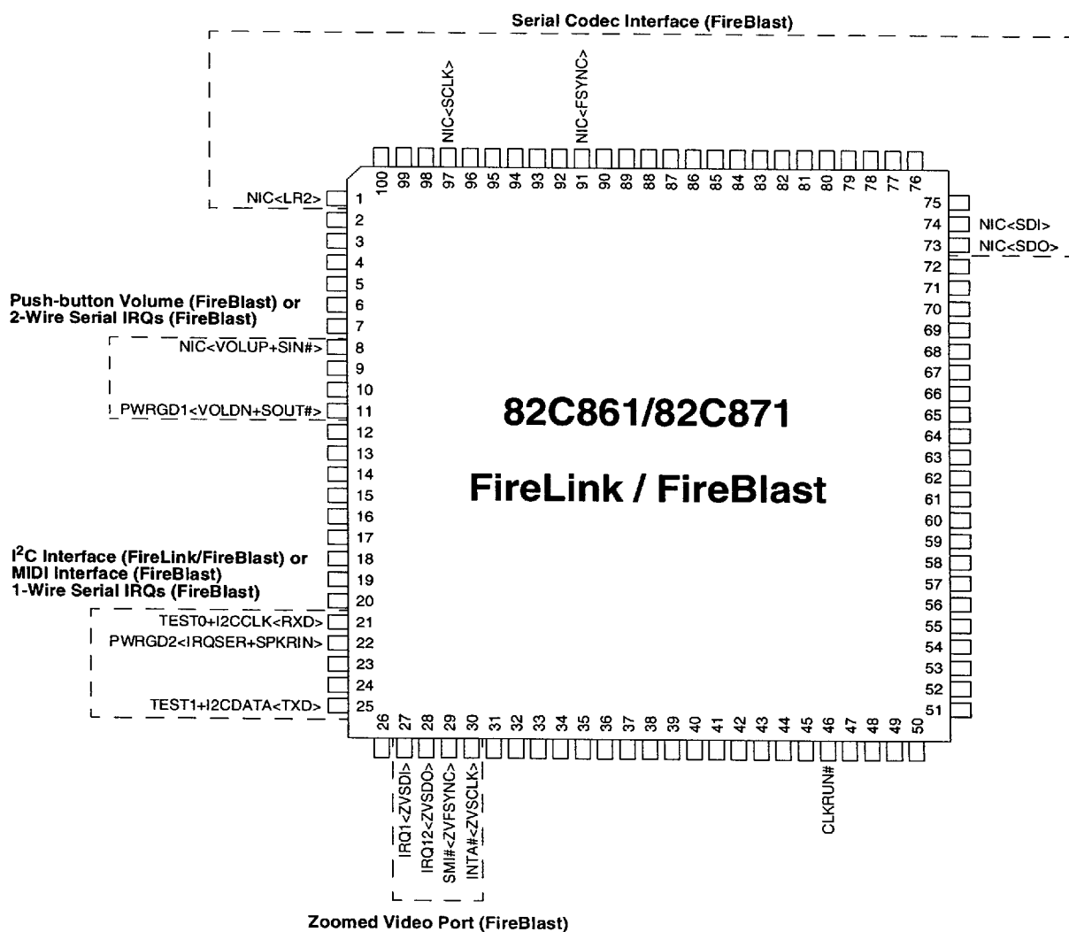
Figure 2-2 Functional Grouping
