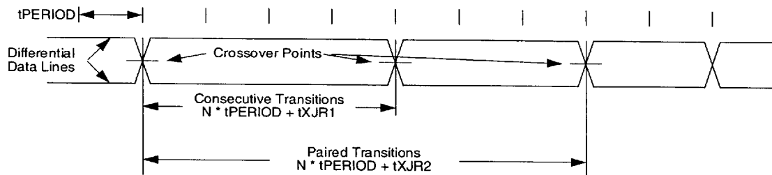
Figure 6-4 Differential Data Jitter
