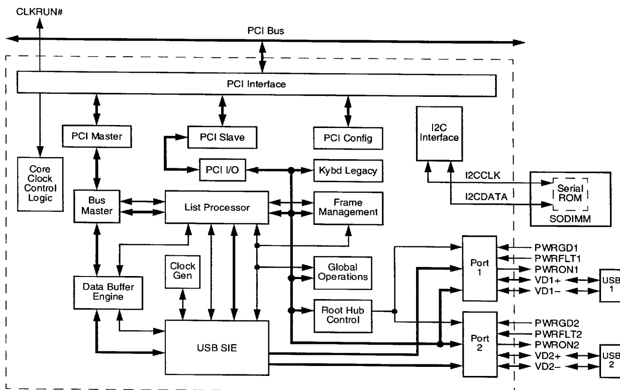
Figure 2-3 FireLink Block Diagram
