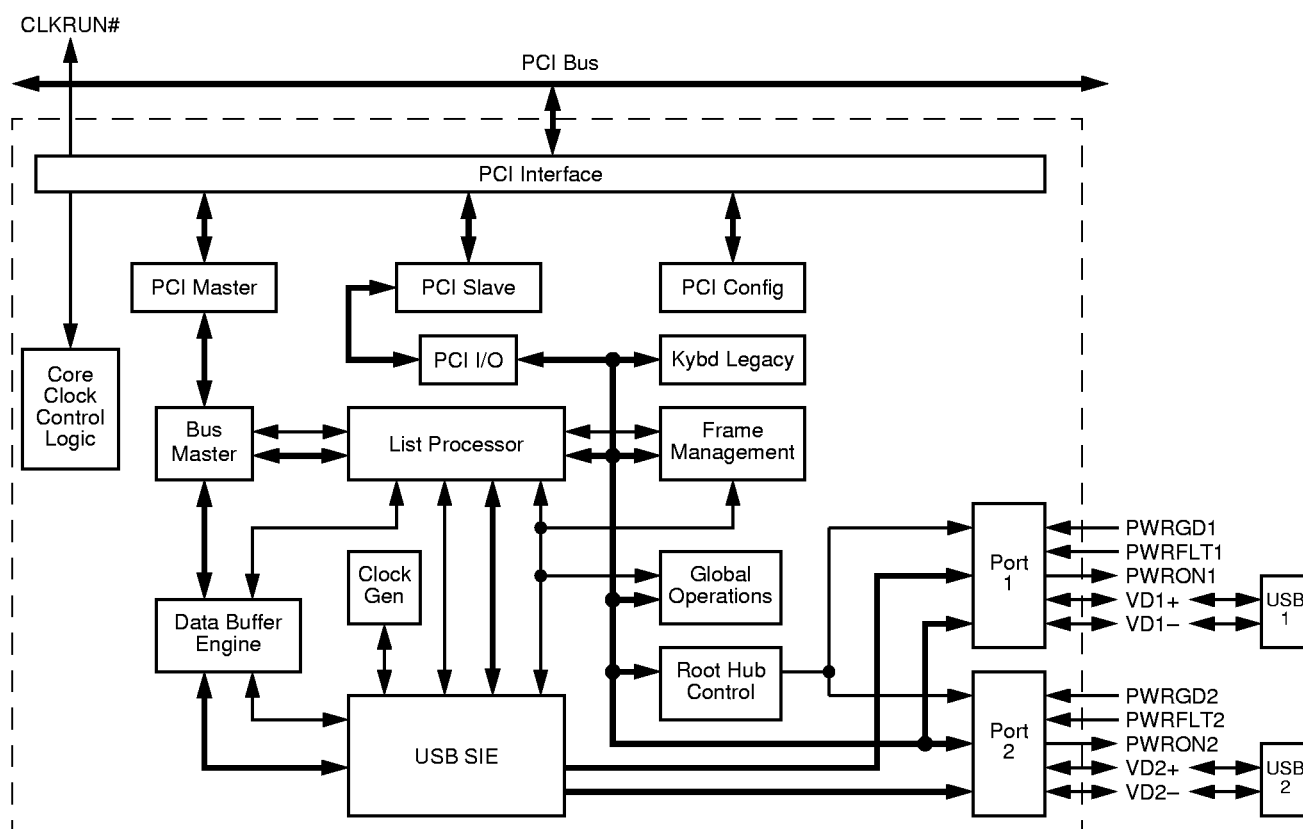
Figure 2-1 FireLink Block Diagram
