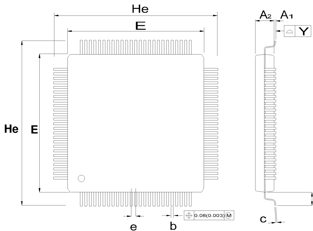
Figure 7-1 100-Pin Low-Profile Quad Flat Pack (LQFP)
