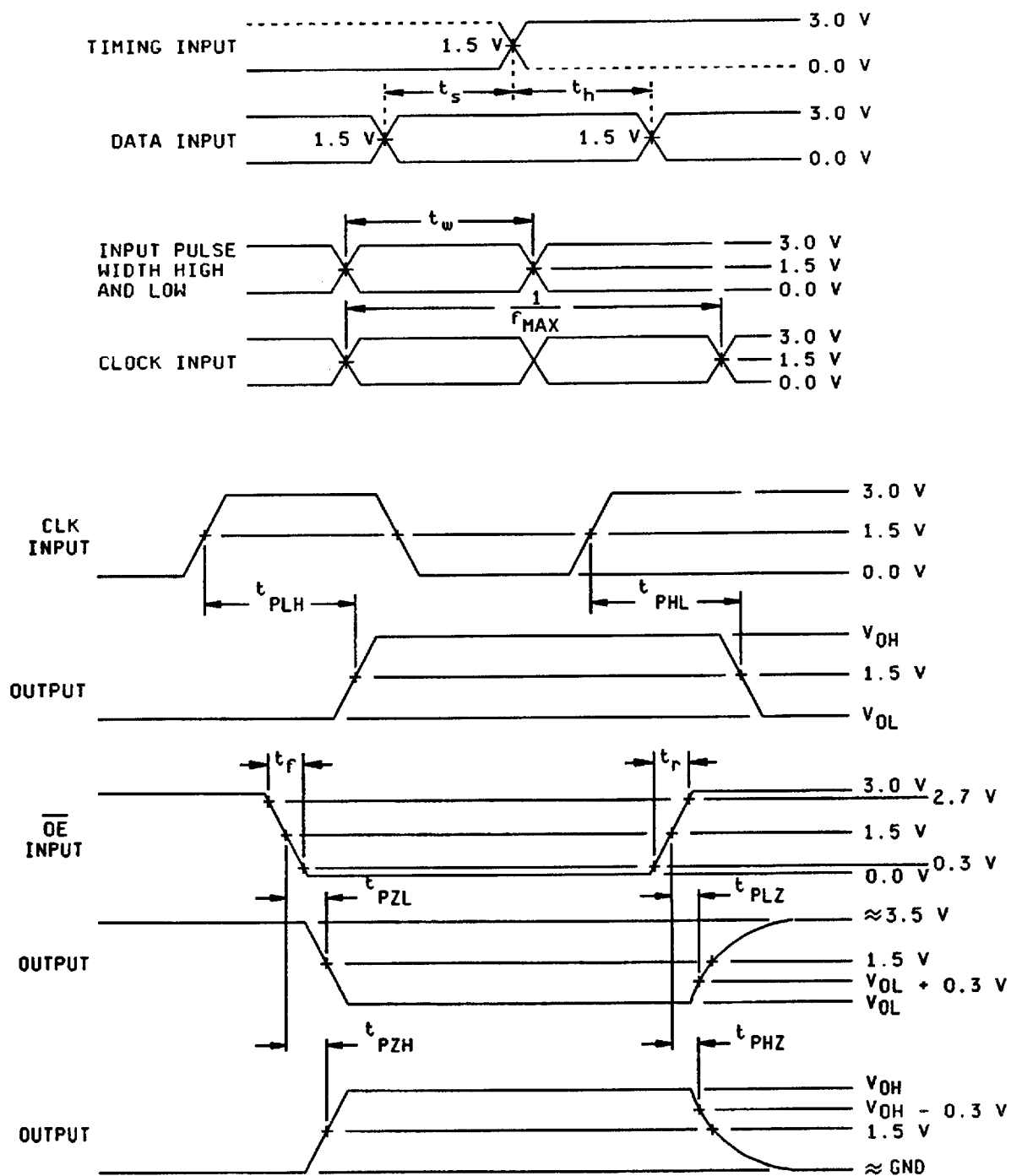
FIGURE 5. Switching waveforms and test circuit
