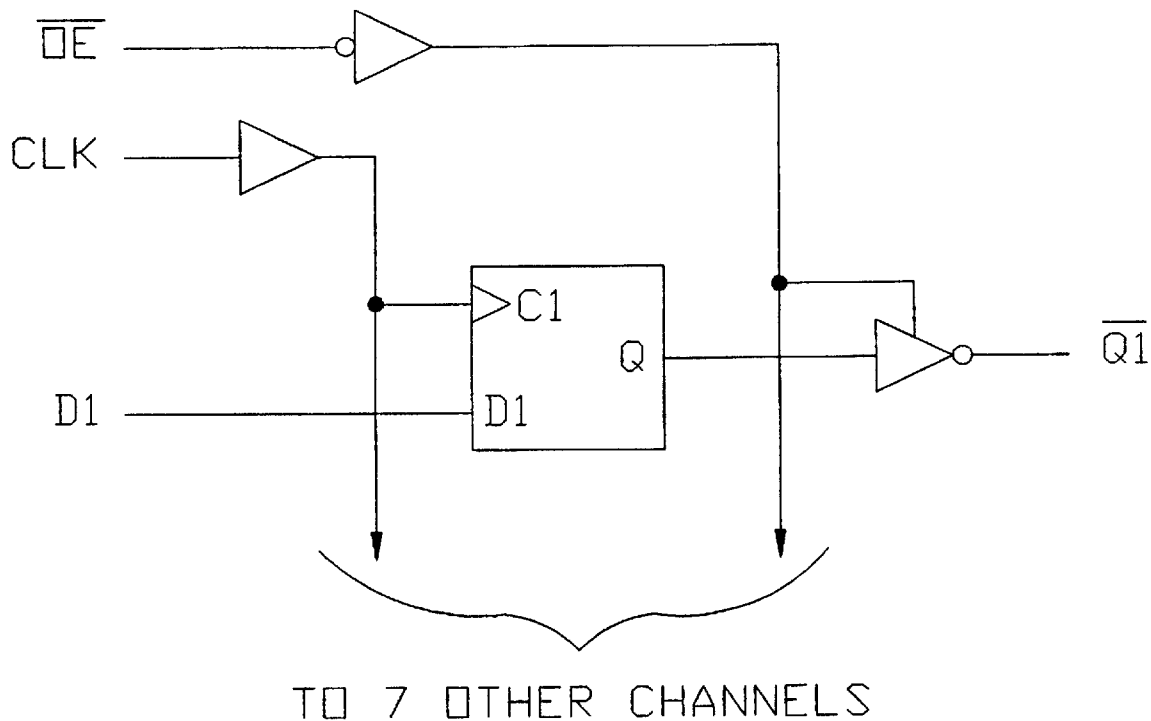
FIGURE 3. Logic diagram.
